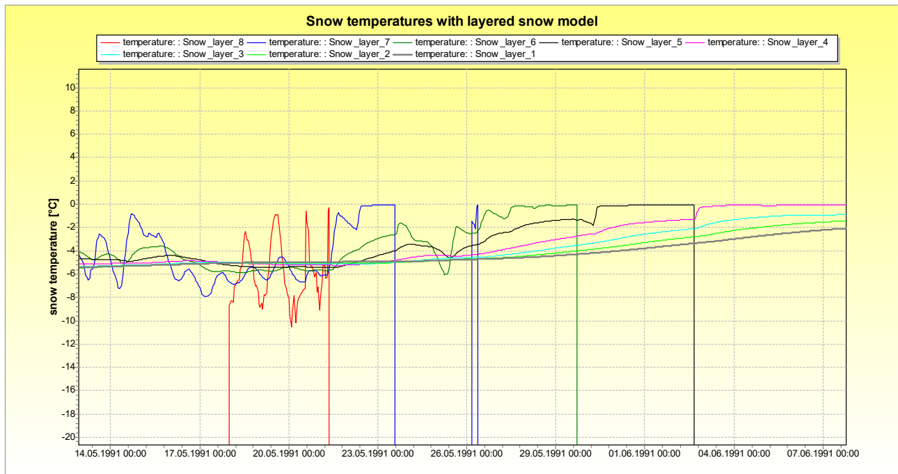
figure 2.27.3.5: snow temperatures for a melting snow pack with up to eight snow layers
