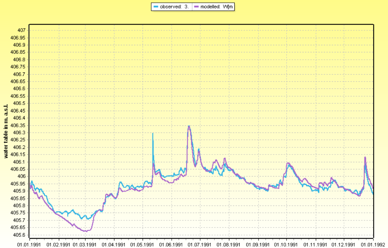
Abbildung 2.19.2: Comparison of modeled (purple) and observed water levels (blue) for lake Zurich without externally read abstraction values (purely modeled)
