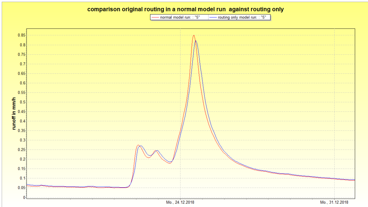
figure 2.17.3.4: Comparison between routing results for a normal model run (red) and a routing only model run (blue) with different roughness parameters; December 2018 flood event; Gauge Kander/Hondrich (491km 2 )
