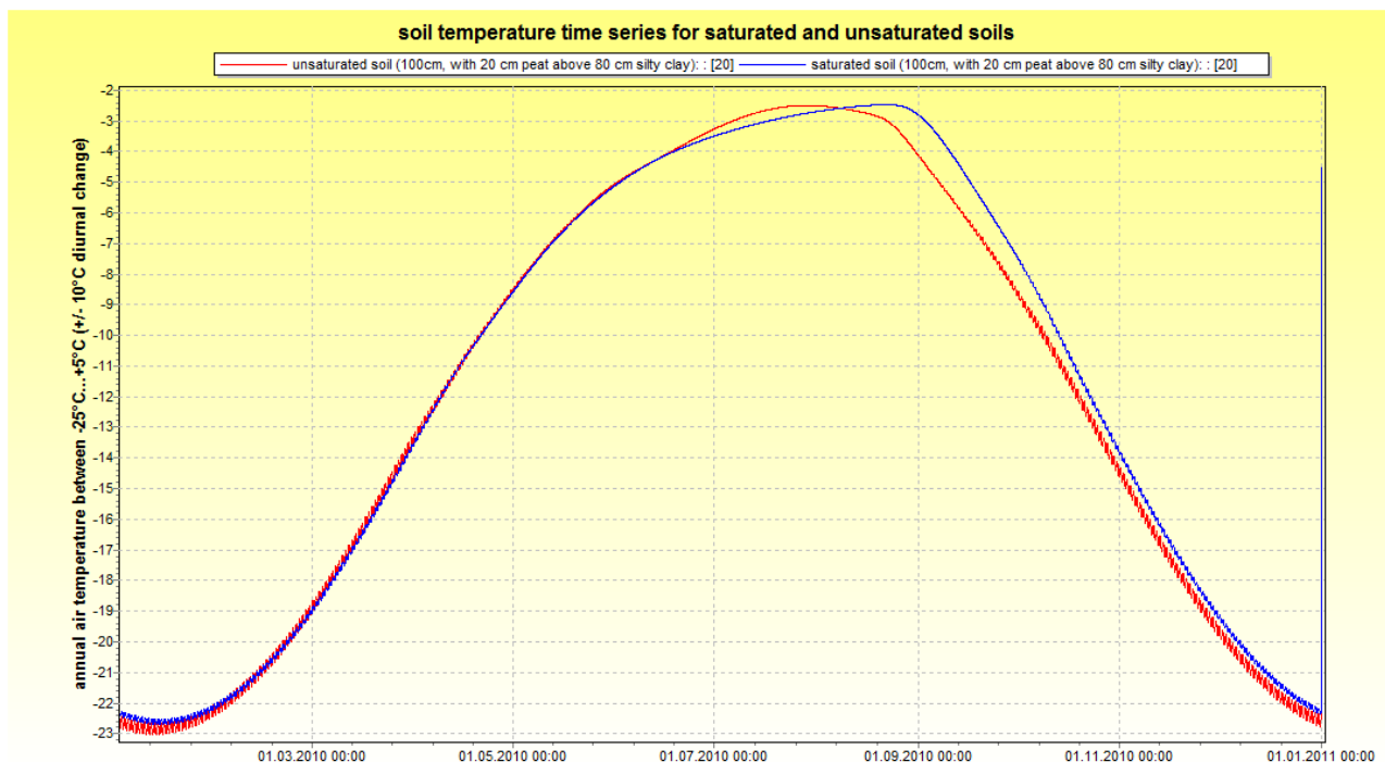
figure 2.25.8.15: Comparison of soil temperatures in 100 cm depth for a saturated (blue) and unsaturated (red) soil with 20 cm peat (porosity 0.8) above 80 cm silty clay
