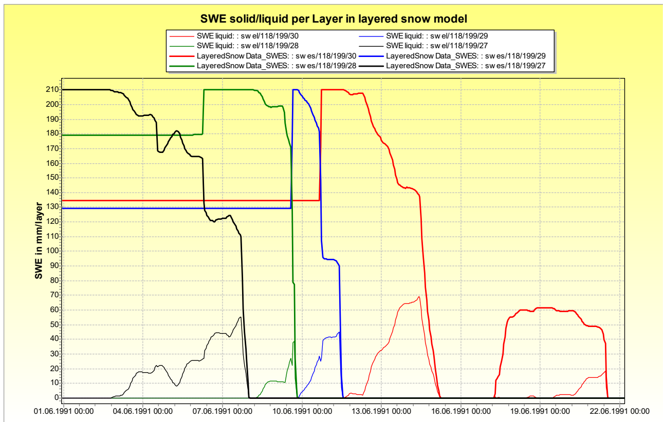
figure 2.27.3.4: Detail of SWE solid and liquid per layer. The thin graphs are the liquid water content.
