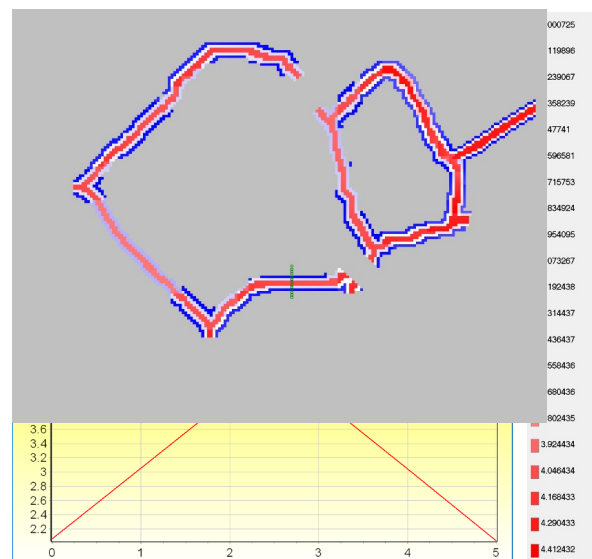
figure 2.29.2.1 IceWedgeLowerLimit (iwdeglo) for the test basin (depth in cross section is between 2 and 4 m below surface)
