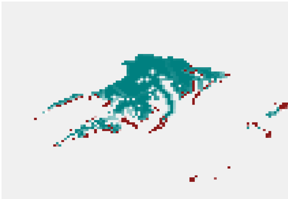
figure 2.22.2.2: Glaciers in the Swiss Alps for 2010
