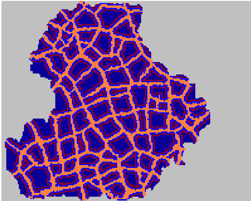
figure 2.26.3.3: All HRUs for a flat arctic tundra basin with typical permafrost structures (low centered polygons)
