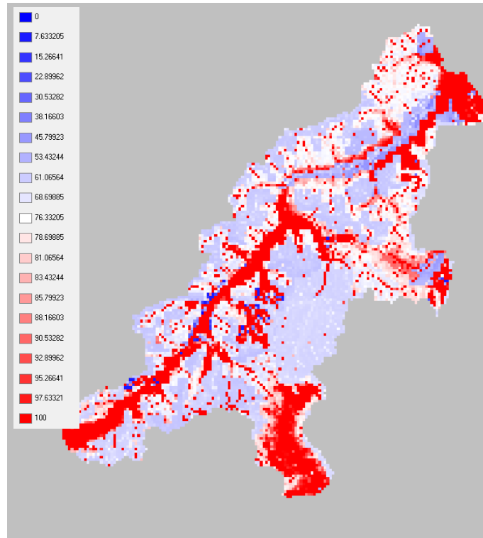
figure 2.14.16.4: actual water content 1991-01-31 as percentage of actual content on field capacity (in %)
