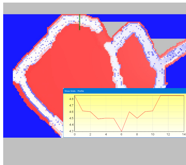
figure 2.29.2.5: DEM after year 1, the cross section shows the decreased soil surface over the degraded ice wedges
