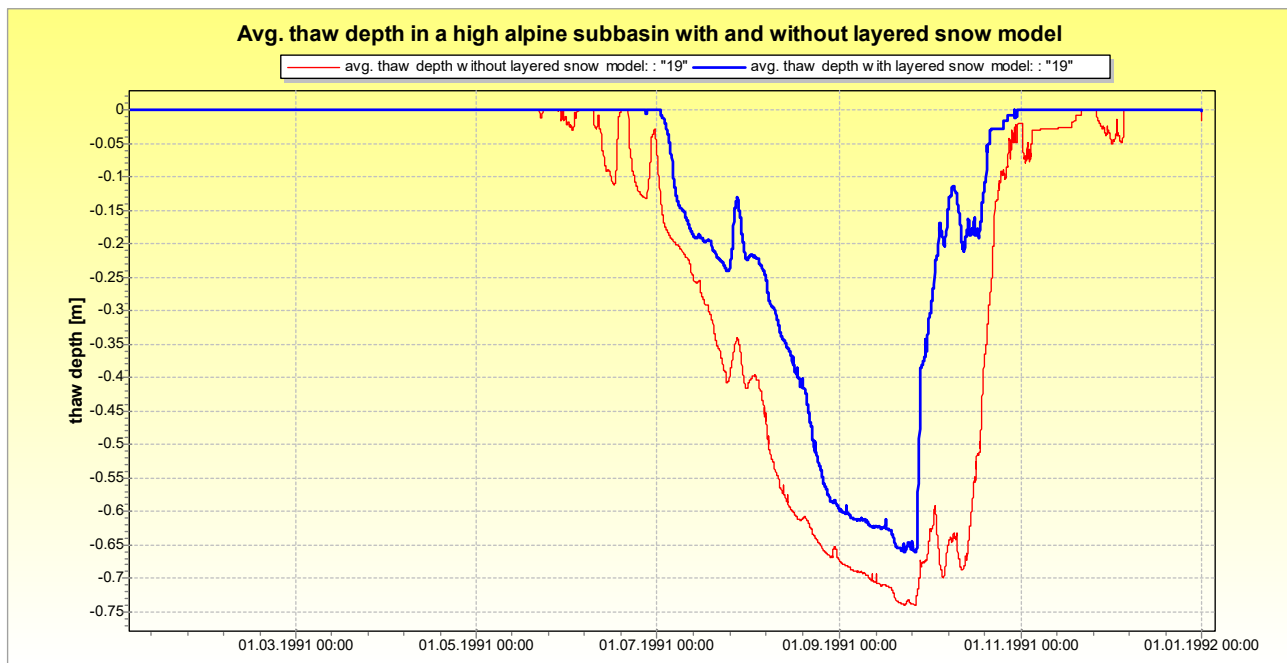
figure 2.27.3.2: average thaw depth for the same high alpine sub basin using layered snow model (blue) and using the conventional snow model (red)
