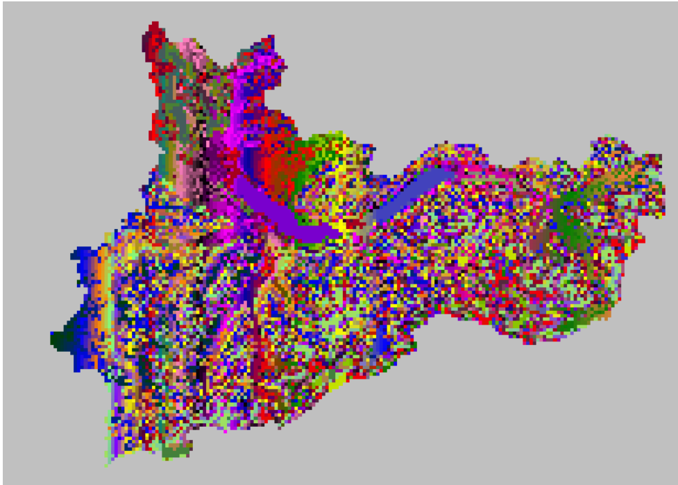
figure 2.26.3.1: HRUs for all cells (basin of the river Aare up Berne, Switzerland, 11826 cells (=2956.5 km 2 ))
