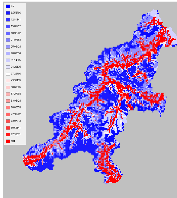
figure 2.14.16.1: Residual water content in minFieldCapacity_mm
