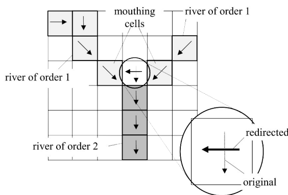
figure 5.1.27.3: flow direction correction at mouths
