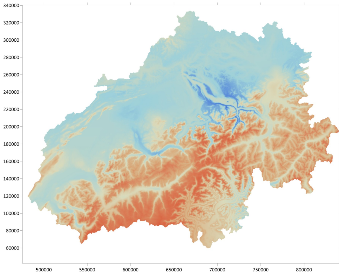
figure 2.3.15.2: Example of relative air humidity interpolation results for all Swiss river basins, interpolated independently of each other but with smooth shifts between regions
