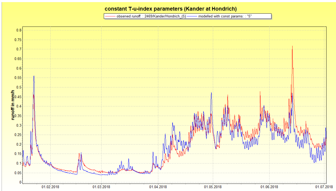
figure 2.9.8.2: Comparison of observed runoff (red) vs. modelled runoff (blue) for default static snow melt parameters
