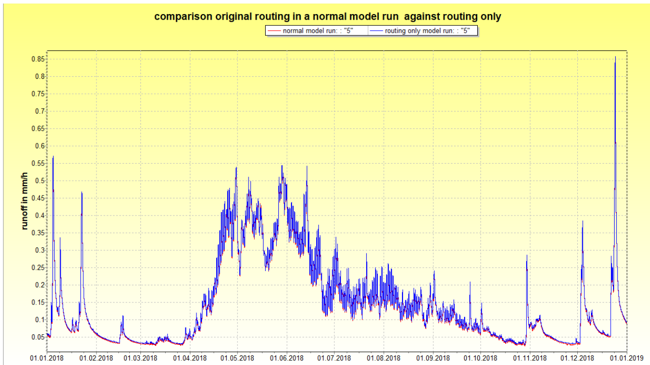
figure 2.17.3.1: Comparison between routing results for a normal model run (red) and a routing only model run (blue) with identical parameters; 2018, Gauge Kander/Hondrich (491km 2 )
