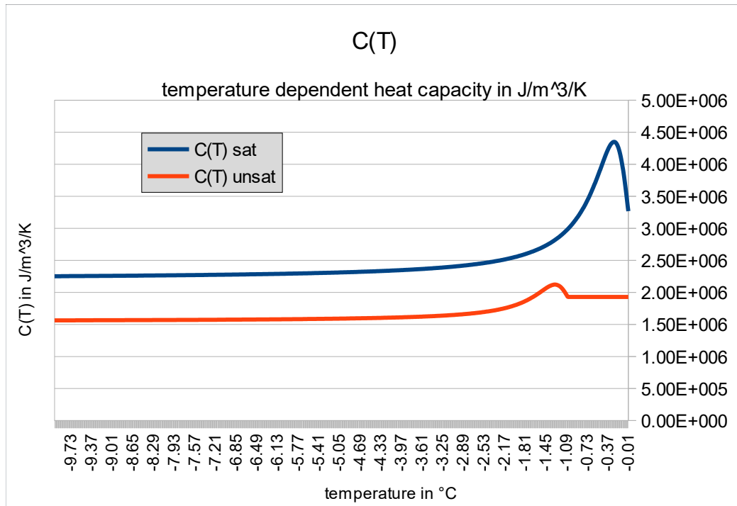
figure 2.25.5.2: The change in effective heat capacity of a freezing/thawing soil ( \Theta_s = 0.5 and \Theta_r = 0.1 ) for saturated ( \Theta = 0.5 and unsaturated ( \Theta = 0.18 ) conditions.
