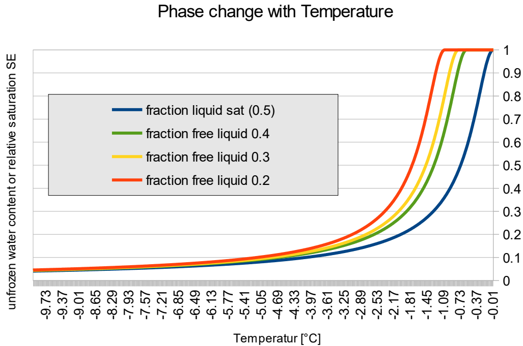
figure 2.25.2.1: Change in the fraction of liquid water, S_E , during temperature change in a sandy loam soil ( \alpha=2 , n=2 , m=0.5 ). (temperatures are negative from -10 to 0°C)
