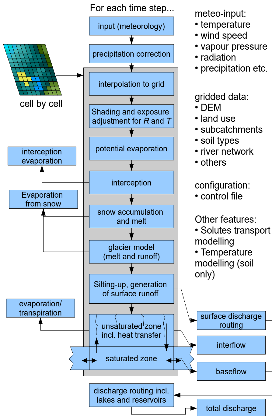
figure 2.1.1: model structure of WaSiM
