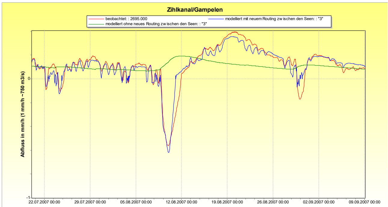
figure 2.19.9.2: example for flow reversals between lakes Bielersee and Neuenburgersee due to the new abstraction rule as hydraulic connection
