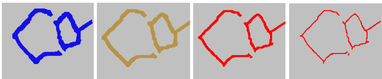
figure 2.29.2.3: Excess ice stack: Level 3, 9, 14 and 17 with 45.9, 41.8, 183.6 and 183.6 mm WE
