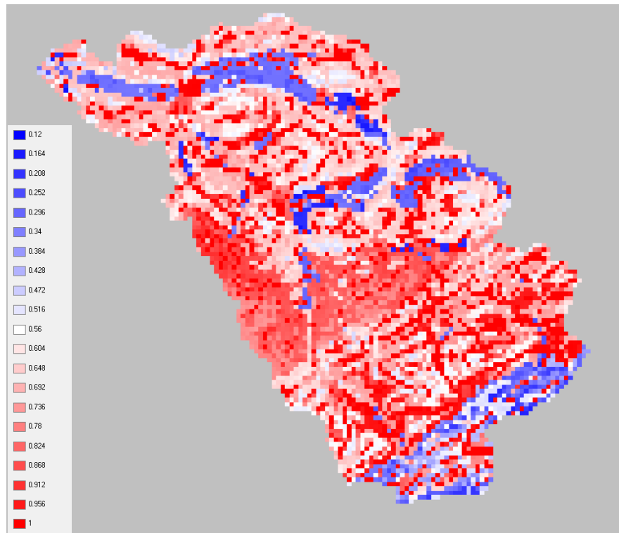
figure 2.14.18.2: spatial distribution of relative soil moisture for January, 7th, 1991, Thur basin
