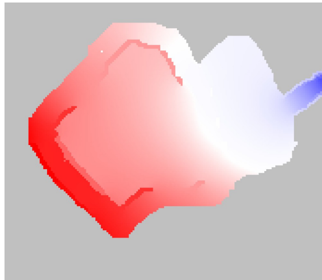
figure 2.29.2.4: original DEM (almost) without any channels
