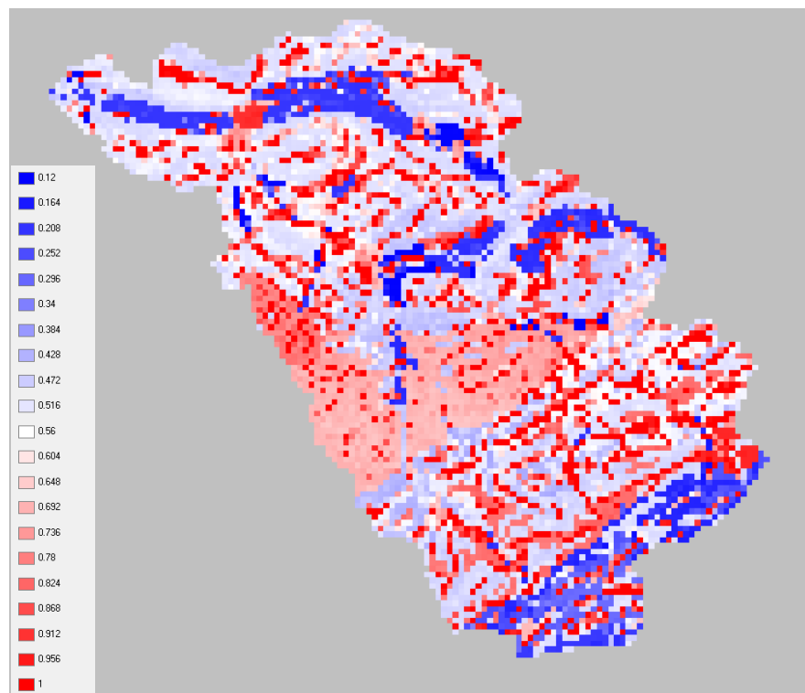
figure 2.14.18.3: spatial distribution of relative soil moisture for January, 31st, 1991, Thur basin
