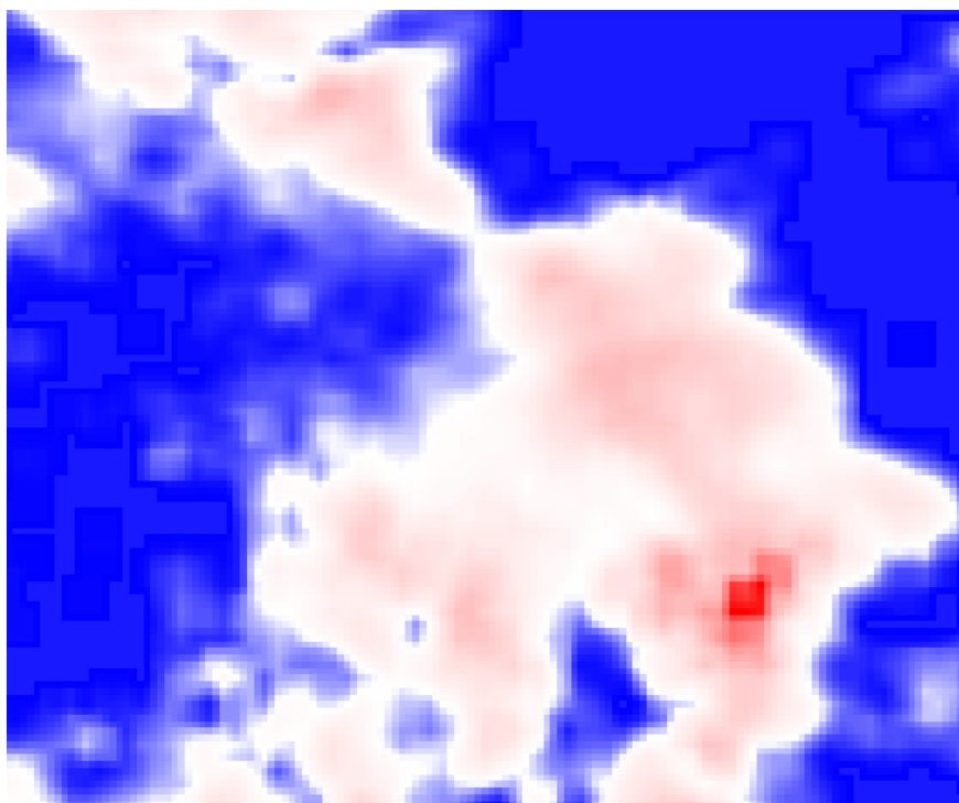
figure 2.3.9.2: interpolated region of interest, mapped to precipitation values
