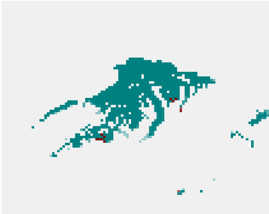
figure 2.22.2.1: Glaciers in the Swiss Alps (center: Aletschgletscher) for 1996
