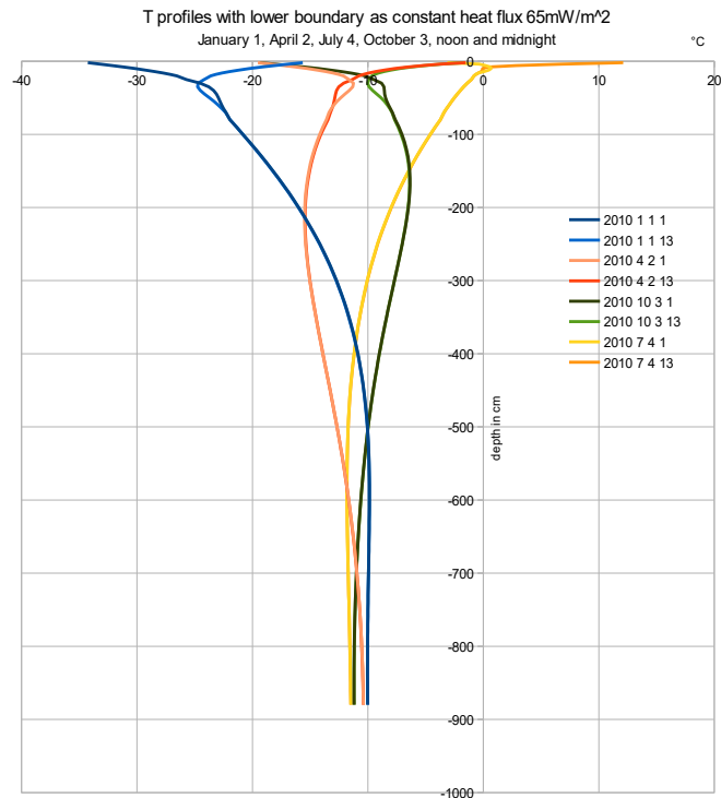
figure 2.25.8.12: T-profile with initial T of -9.478^{\circ}\text{C} and constant heat flux of 65\text{mW/m}^2 as lower boundary condition
