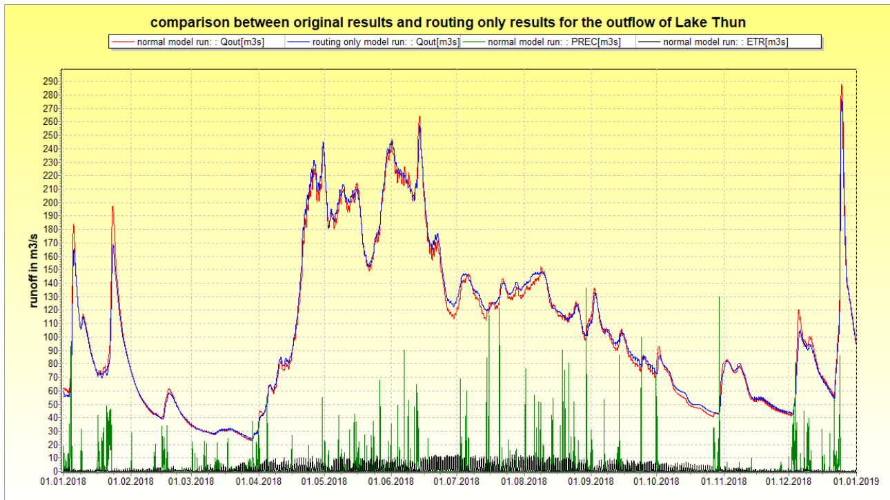
figure 2.17.3.5: comparison between original model run and routing only model run for the outflow of Lake Thun, 2018; red=normal model run, blue=routing only model run; green=precipitation from the lake surface, black = evaporation from the lake surface
