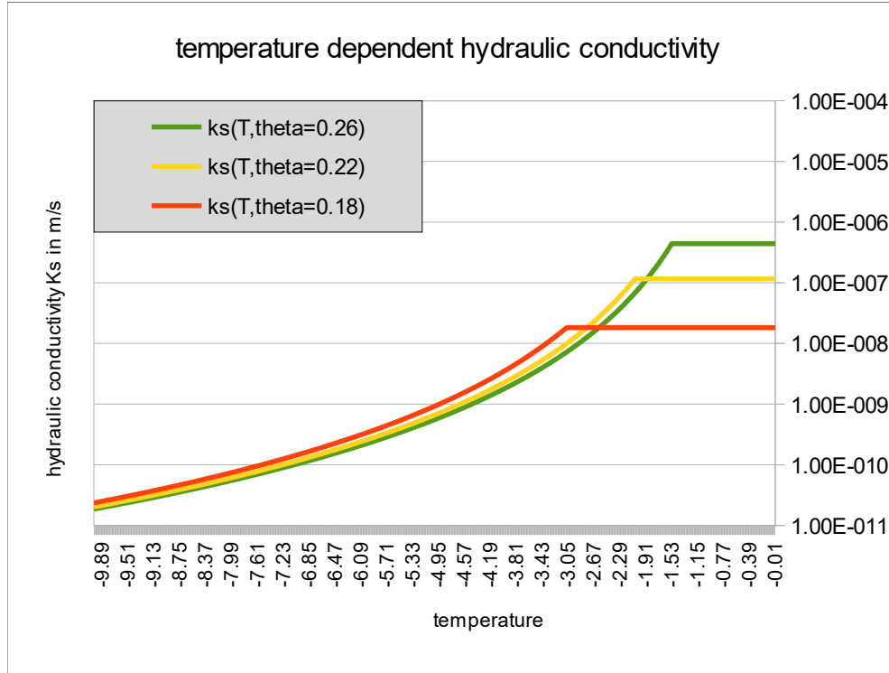
figure 2.25.4.3: Effective unsaturated hydraulic conductivity using an exponential function and a variable ks -value based on equation (2.24.8c)
