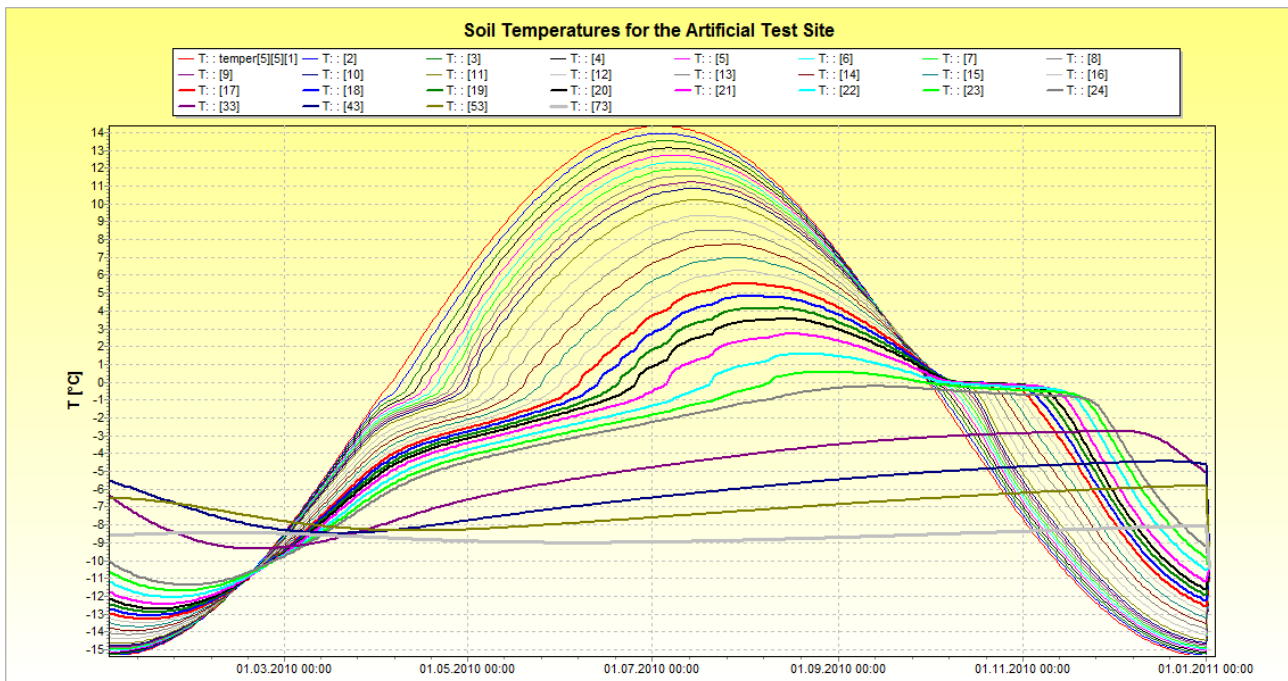
figure 2.25.8.4: soil temperatures for the artificial test site (upper horizon: 20 cm of organic material, modelled in 10 layers of 2 cm each, then 10 cm layers follow; profile has a total depth of 10 m --> the fat, dark grey graph is at around 7 m)
