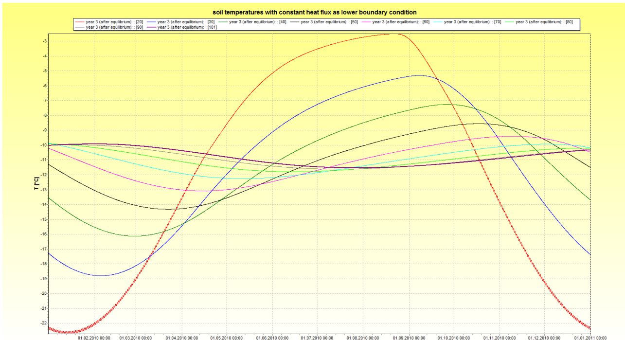
figure 2.25.8.10: soil temperatures as time series for constant heat flux of 65 \text{ mW/m}^2 lower boundary condition (red=0.7m, blue = 1.7m, green = 2.7m, black = 3.7m etc. down to 8.8m for violet)
