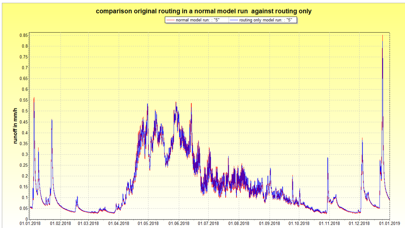
figure 2.17.3.3: Comparison between routing results for a normal model run (red) and a routing only model run (blue) with different roughness parameters; 2018, Gauge Kander/Hondrich (491km 2 )
