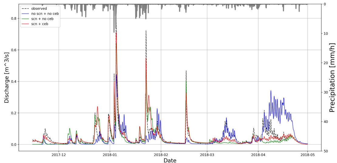
figure 2.10.3.2: Comparison of simulated and measured discharge data during validation run in winter 2017/18
