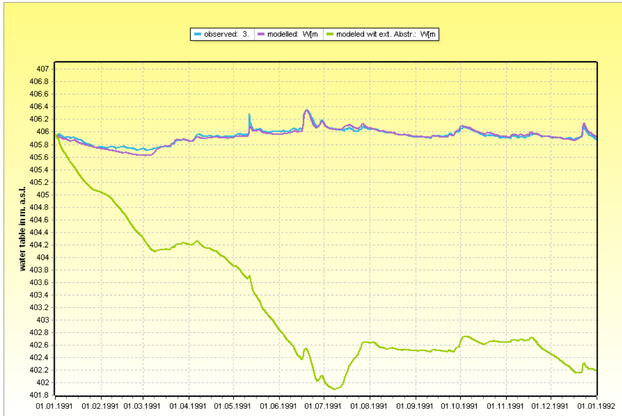
Abbildung 2.19.4: Comparison of modeled and observed water tables for lake Zurich without (purple) and with externally read abstraction values (green)
