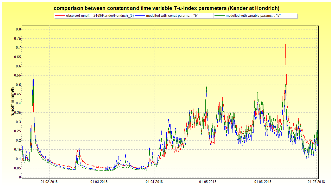
figure 2.9.8.1: comparison of modeled runoffs versus observed runoff (red) for blue=constant T-u-index parameters and green = temporally variable parameters
