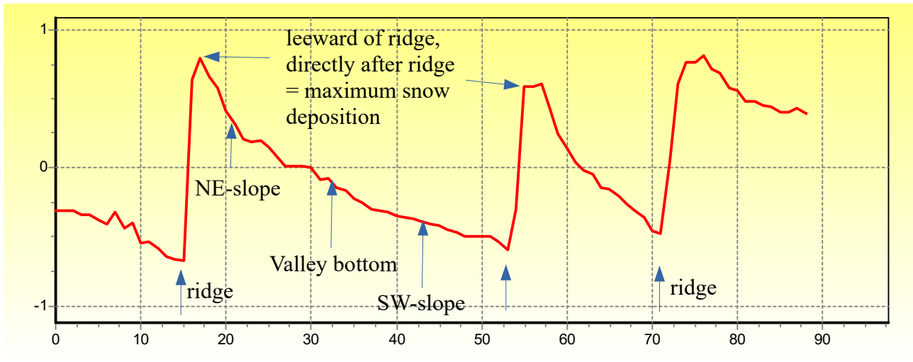
figure 2.9.3.3 profile A-B (see figure 2.9.3.2) for a SW main wind direction
