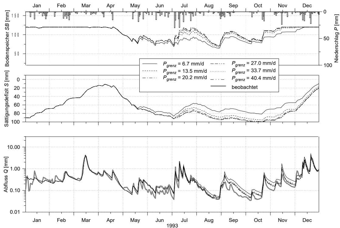
figure 4.15.5: Impact of the threshold precipitation intensity P_{\text{grenz}} for generating macro pore drainage on (a) soil moisture, (b) saturation deficit and (c) runoff; without capillary rise/reflow from interflow into soil storage ( r_k = 0.0 ); Wernersbach, Saxonia, 4.6 km 2 , 365 to 465 m ü.M., daily time steps for 1993; “Abfluss”=discharge, “Sättigungsdefizit”=saturation deficit, “Bodenspeicher”=soil storage, “beobachtet”=observed
