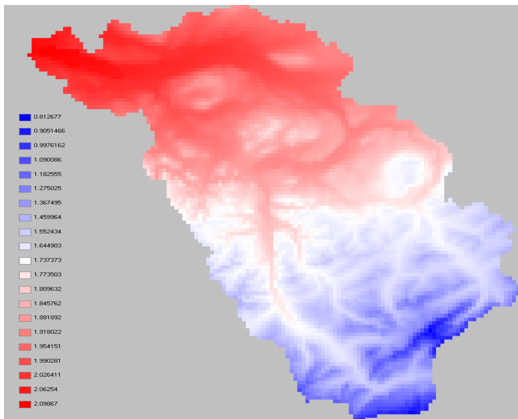
figure 2.3.1.2: example for EDR interpolation for the same data as in figure 2.3.1.1
