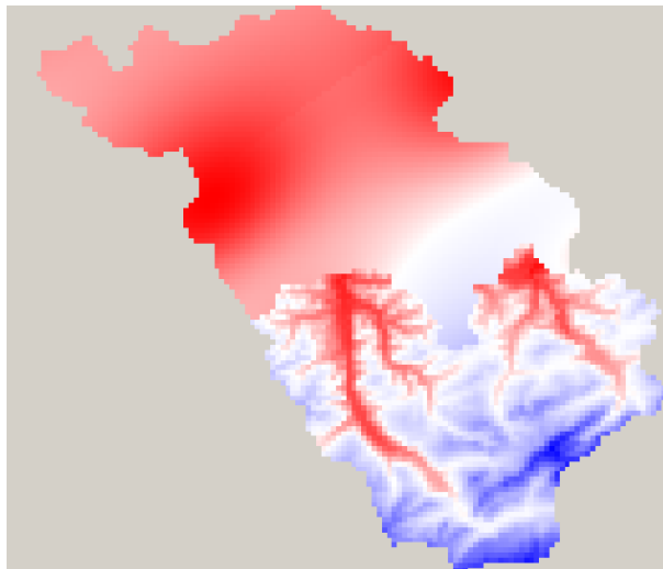
figure 2.3.13.4: interpolation results for IDW (North) and EDR (South) without smooth transition
