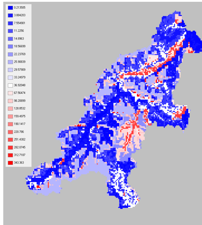
figure 2.14.16.2: Maximum usable field capacity in mm
