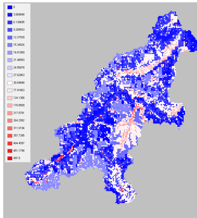
figure 2.14.16.3: actual field capacity 1991-01-31 in mm
