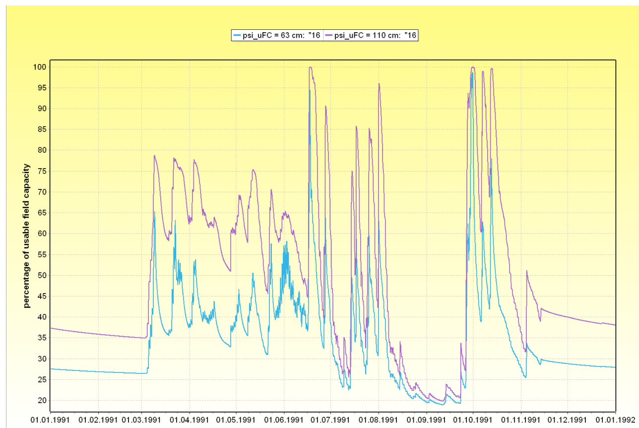
Abbildung 2.14.2: Percentage of usable field capacity for subbasin 16 of the river Inn for different suction pressure thresholds
