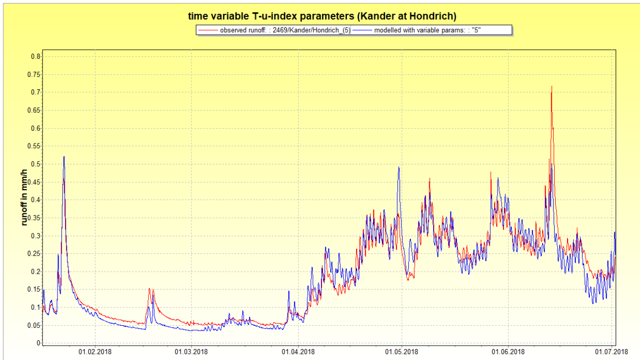
figure 2.9.8.3: Comparison of observed runoff (red) vs. modelled runoff (blue) for temporally variable snow melt parameters
