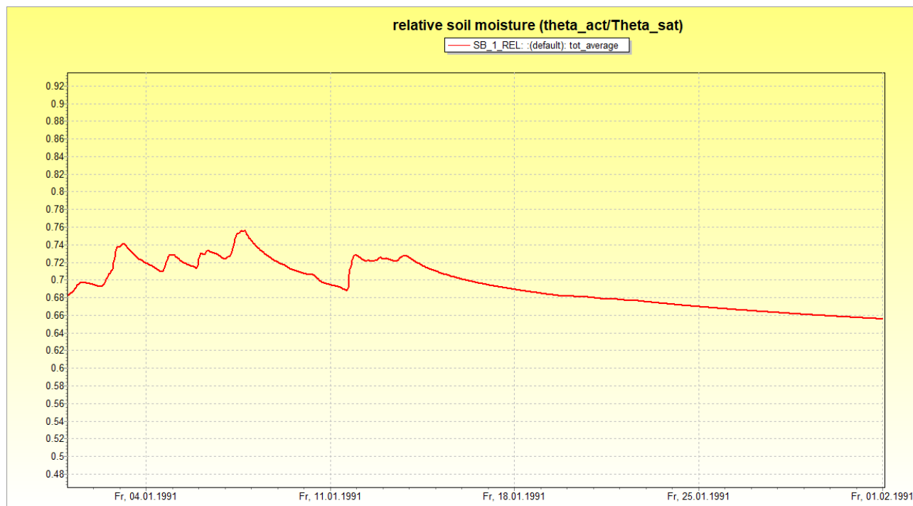
figure 2.14.18.1: statistics for relative soil moisture for the river Thur basin, January 1991
