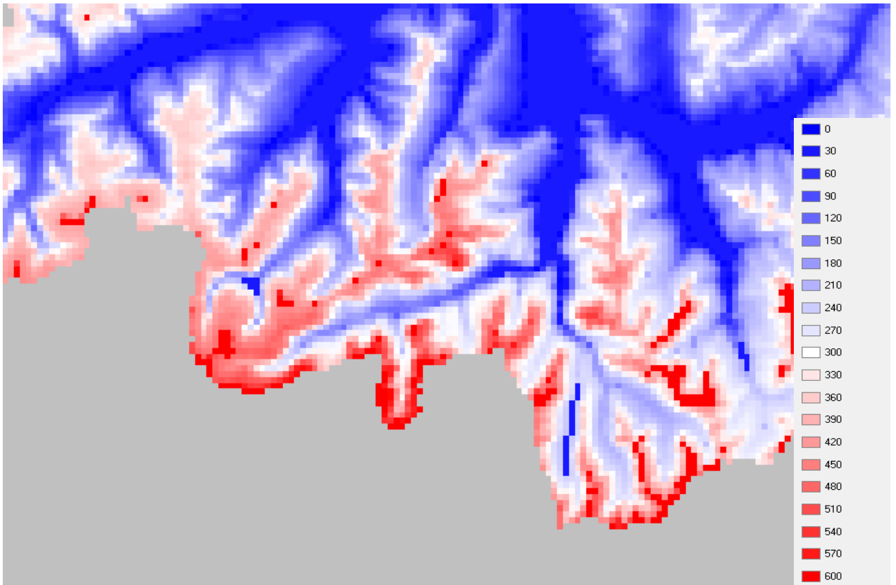
figure 2.9.4.1: snow distribution pattern without slides (in mm SWE)
