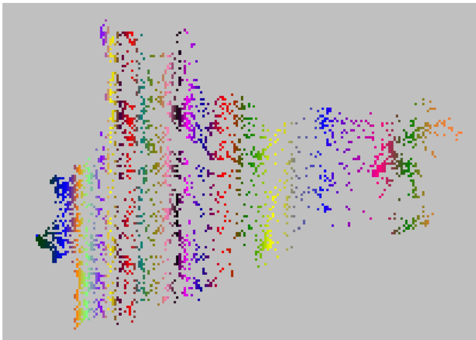
figure 2.26.3.2: HRU master cells (basin of the river Aare up Berne, Switzerland, 2426 cells)
