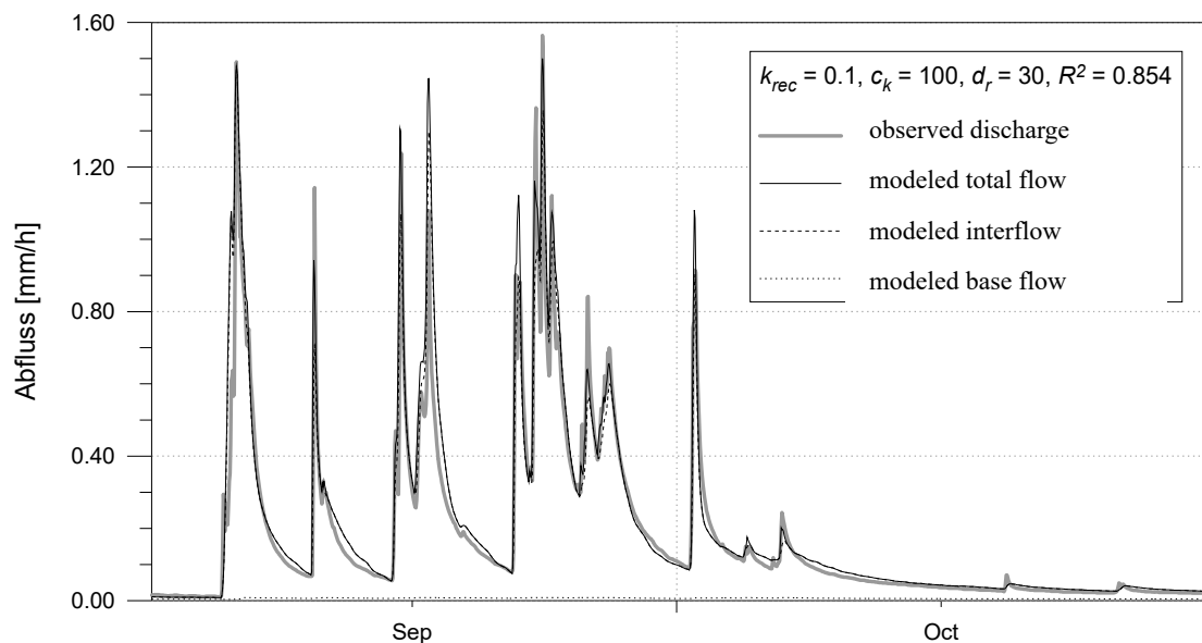
figure 4.16.3.6: Modeled runoff using model version 2 for the Rietholzbach catchment, k_{rec} = 0.1 , d_r = 30
