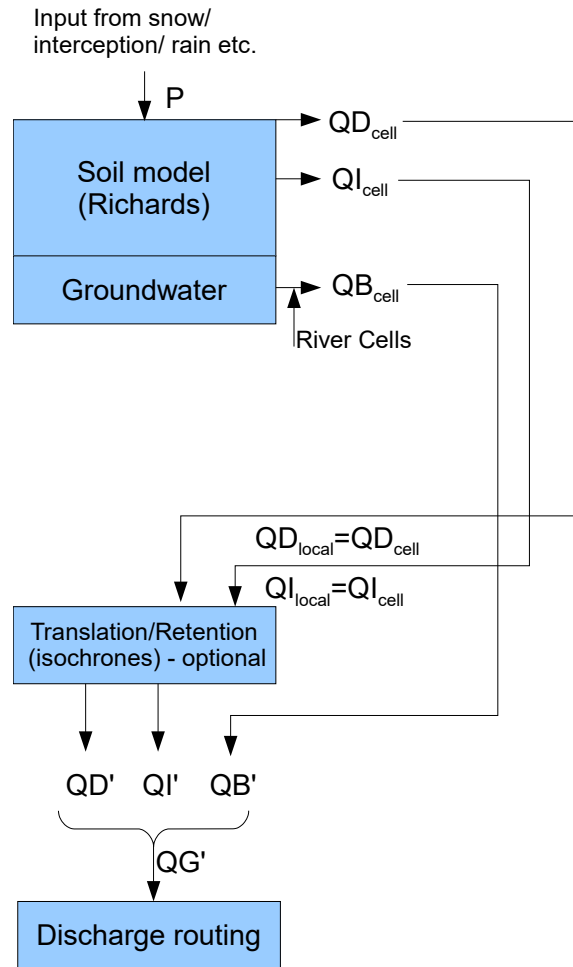
figure 2.13.2.1: Flow chart for traditional soil- and routing modelling (prior to version 8.1.01 and without silting-up and surface routing since version 8.1.01)
