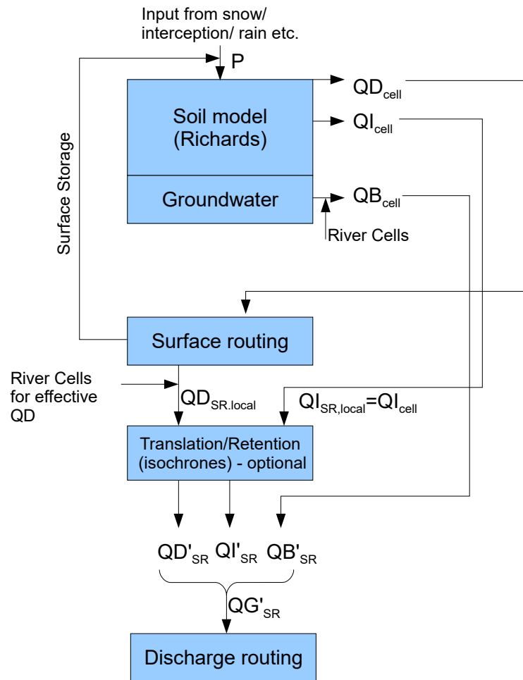
figure 2.13.2.3: Flow chart for soil- and routing modelling including surface routing but without silting-up
