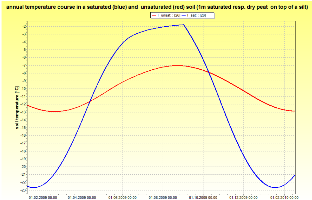
figure 2.25.8.16: temperature time series in a saturated (blue) and unsaturated (red) soil in 1m depth; the soil has a 1m peat layer on a silt. For dry peat, the groundwater is at about -1.3m. No rain, no snow, no evaporation has been regarded in this experiment, only temperature as given in the examples above
