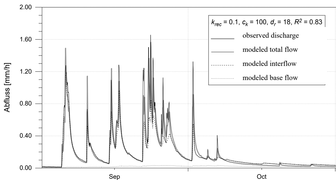
figure 4.16.3.4: Modeled runoff using model version 2 for the Rietholzbach catchment, with interflow, k_{rec} = 0.1
