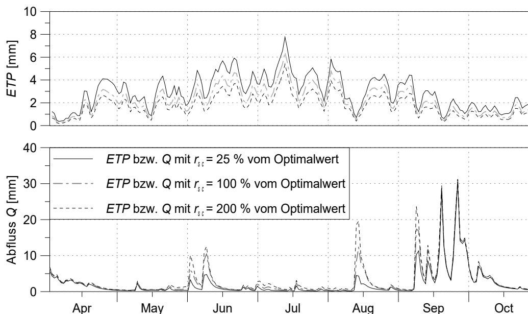
figure 4.15.2.1: model sensitivity on changes in the surface resistances r_s , using results from the Rietholzbach basin for 1984; units of ETP and discharge are in mm/day
