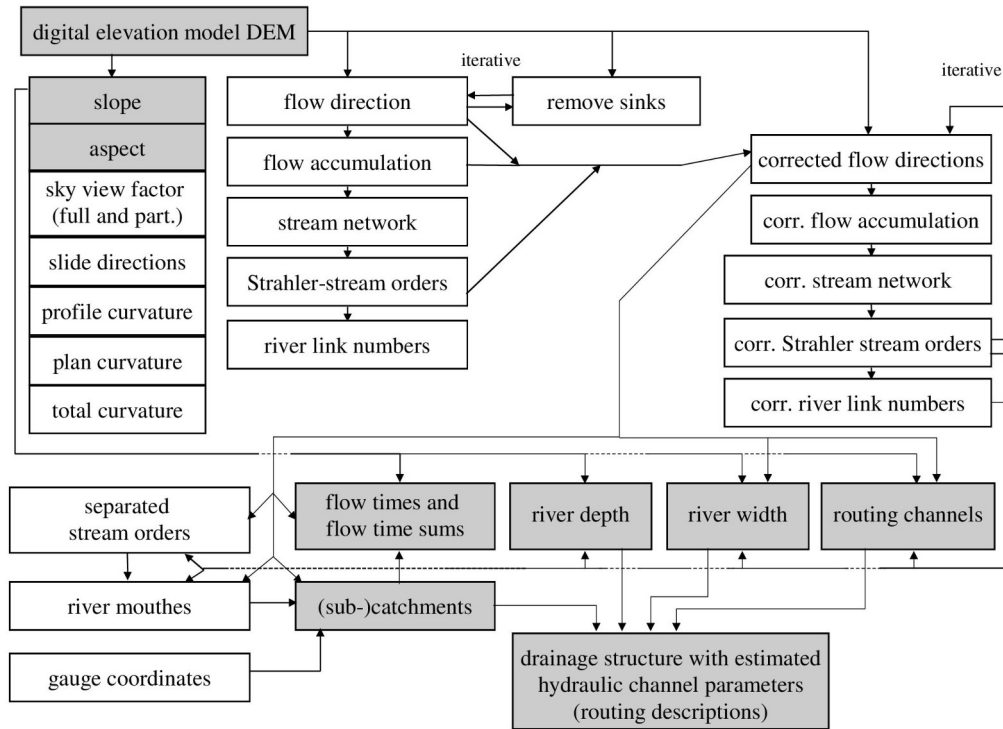
figure 5.1.27.1: topographic analysis of a digital elevation model by TANALYS
