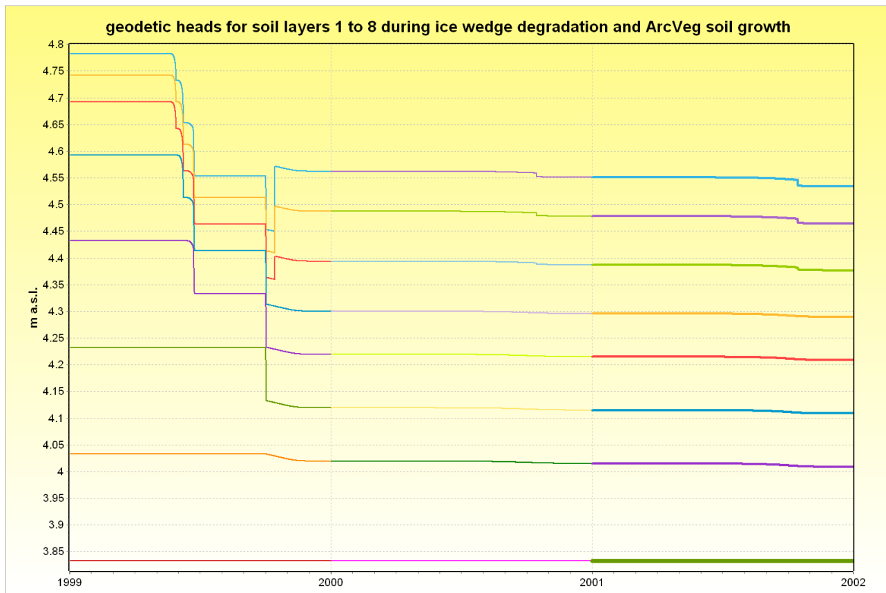
figure 2.29.2.6: time series for geodetic elevation of the uppermost 8 soil layers during ice wedge degradation (1999) and the following stabilization phase (2000 and 2001)
