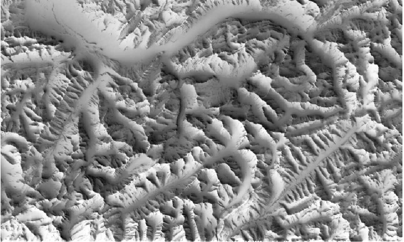
figure 2.9.3.1: Directed sky view factor ( SVF_{dir} ) for 180° to 270° (i.e. SW) for the central Swiss Alps
