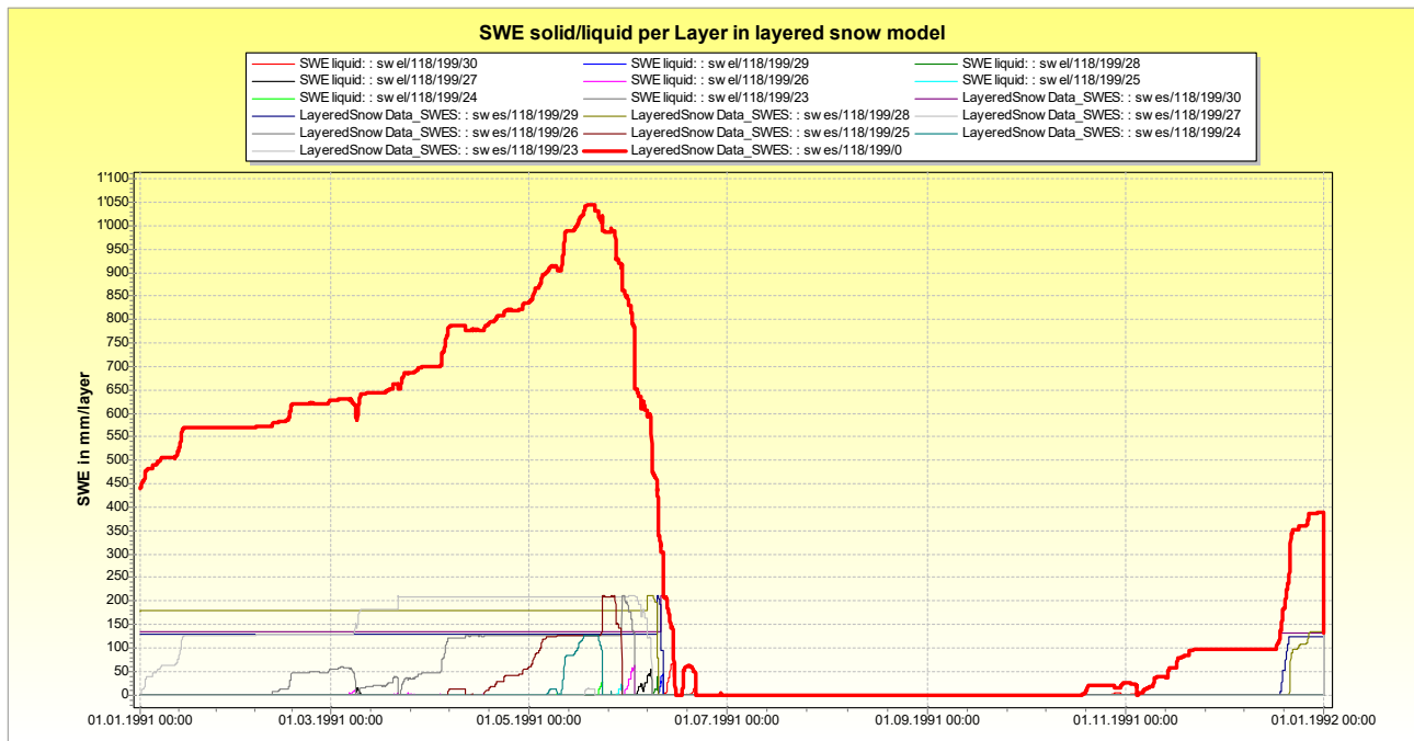
figure 2.27.3.3: SWE solid and liquid per layer as special output time series
