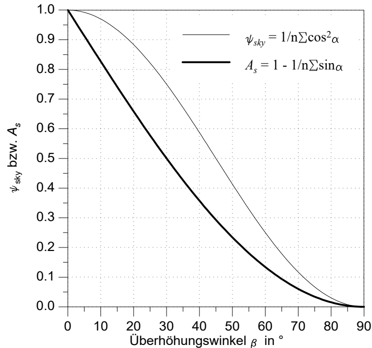
figure 5.1.27.2: ky-view-factor \psi_{sky} and fraction of the sky A_s depending on the horizon overhead angle \beta_h
