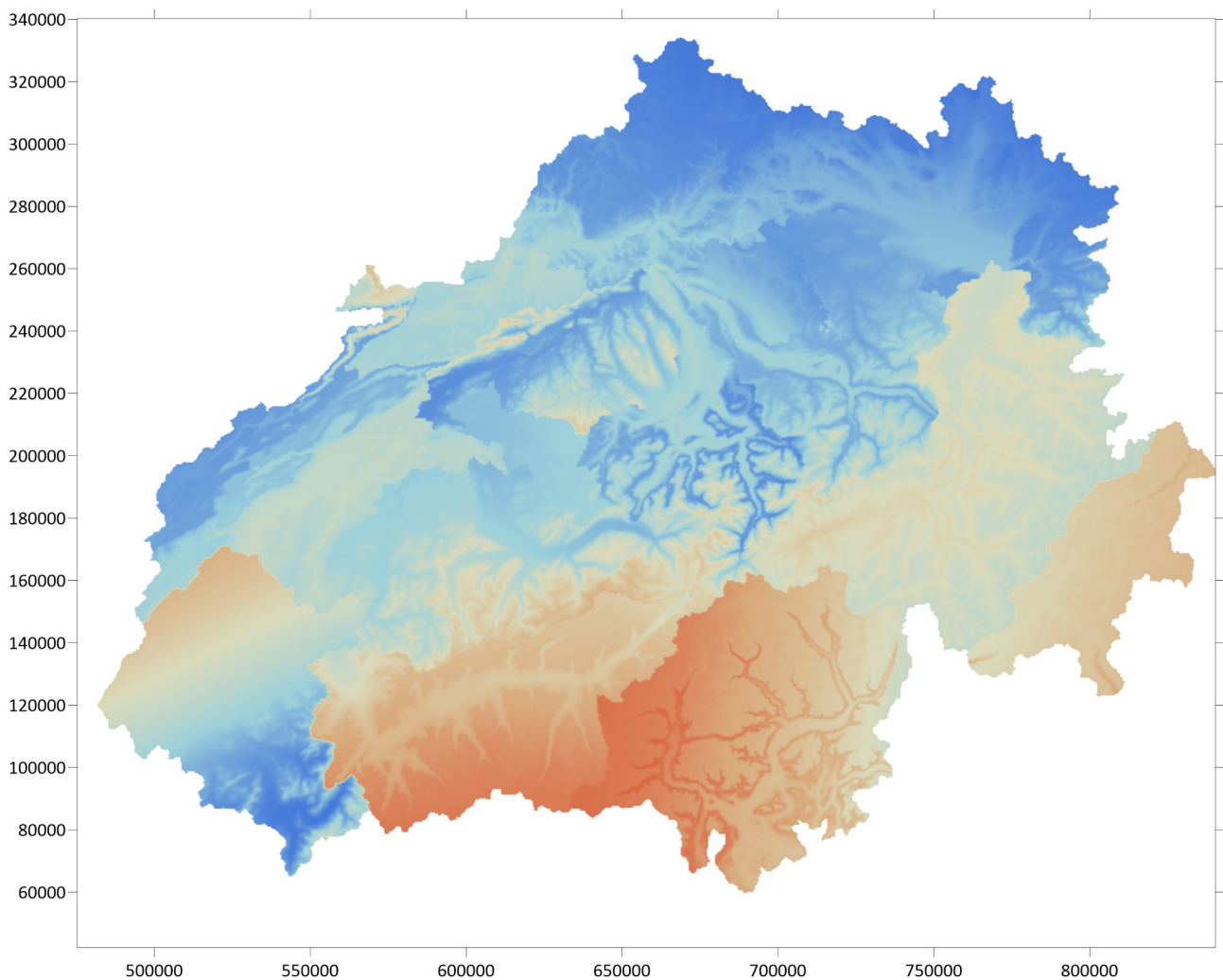
figure 2.3.15.1: Example of relative air humidity interpolation results for all Swiss river basins, interpolated independently of each other
