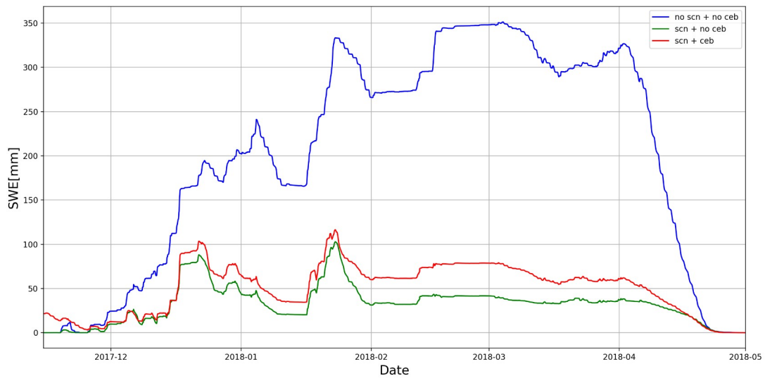
figure 2.10.3.1: Specific SWE stored in the catchment
