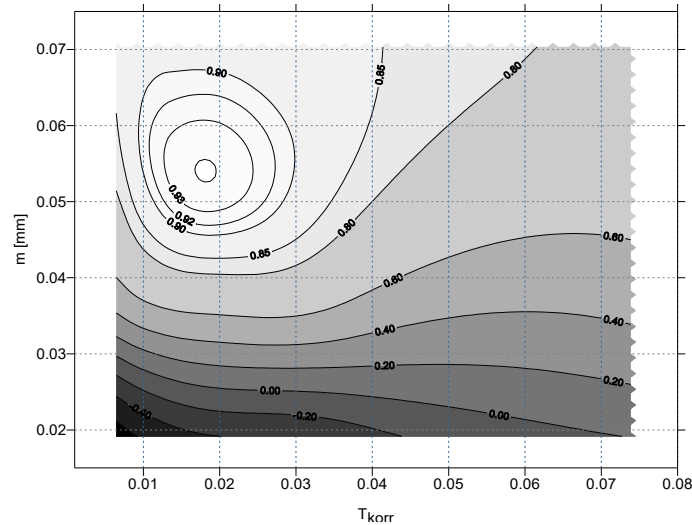
figure 4.15.5.3: distribution of model efficiencies ( R^2 ) as function of T_{korr} and m ; Wernersbach, Saxonia, 4.6 km 2 , 365 to 465 m a.s.l., daily time step, 1993
