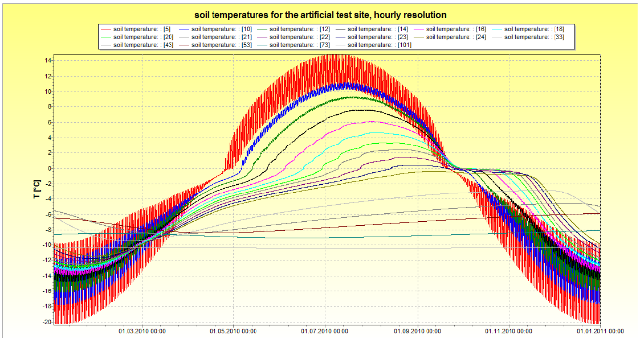
figure 2.25.8.2: soil temperatures for the artificial test site in hourly resolution (shown are temperatures for 10 cm to 110 cm in 10 cm steps and temperatures in 2, 3, 4, 7 and 8.8m)
