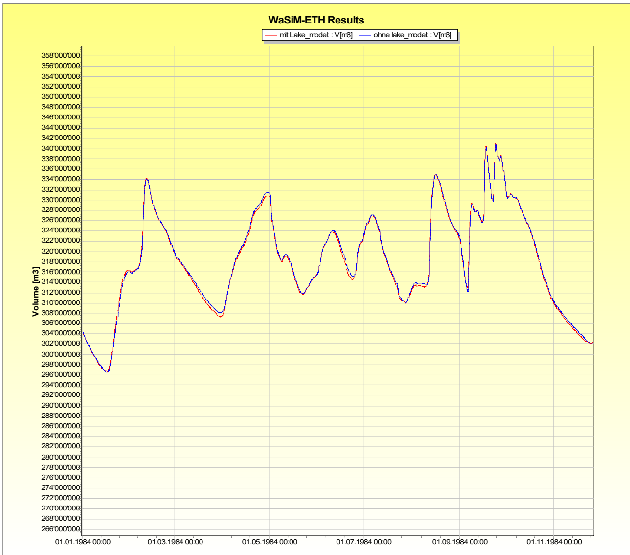
figure 2.19.10.1: comparison of lake volume with the fully integrated lake model and with the simple (routing module only) lake model
