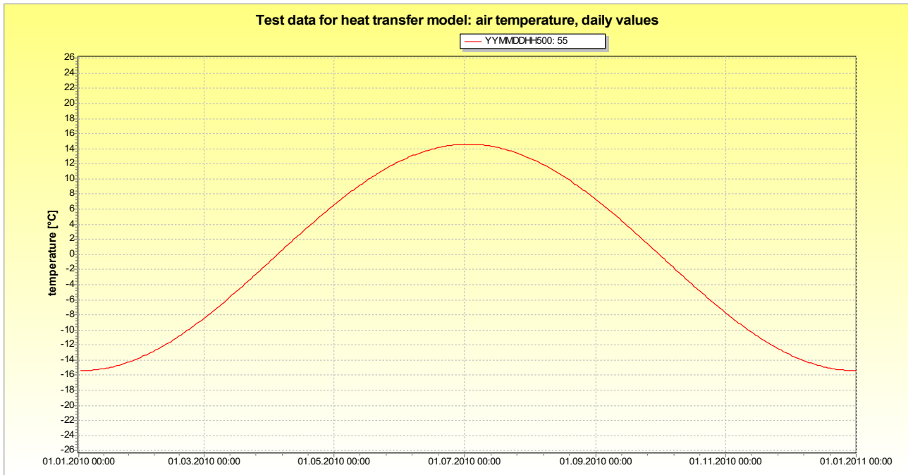
figure 2.25.8.3: temperatures used for heat transfer test data for daily data
