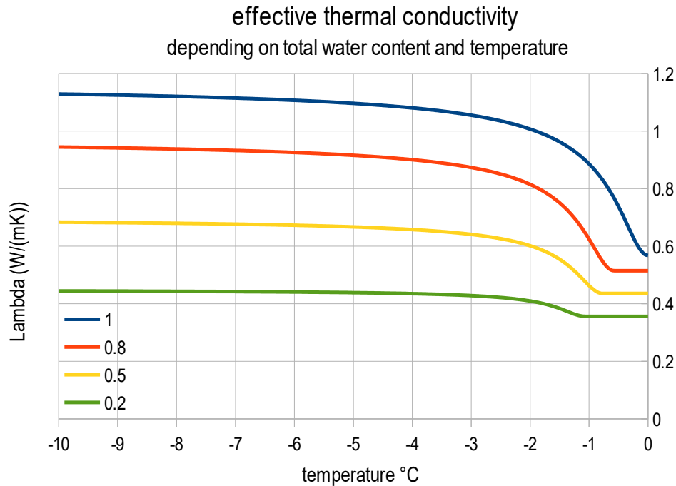
figure 2.25.3.1: Effective thermal conductivity plotted against soil temperature for different relative water contents \Theta_{rel} (1, 0.8, 0.5 and 0.2)
