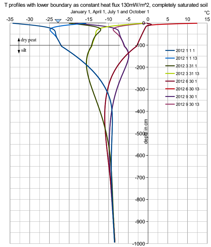
figure 2.25.8.17: T-profiles for saturated soil
