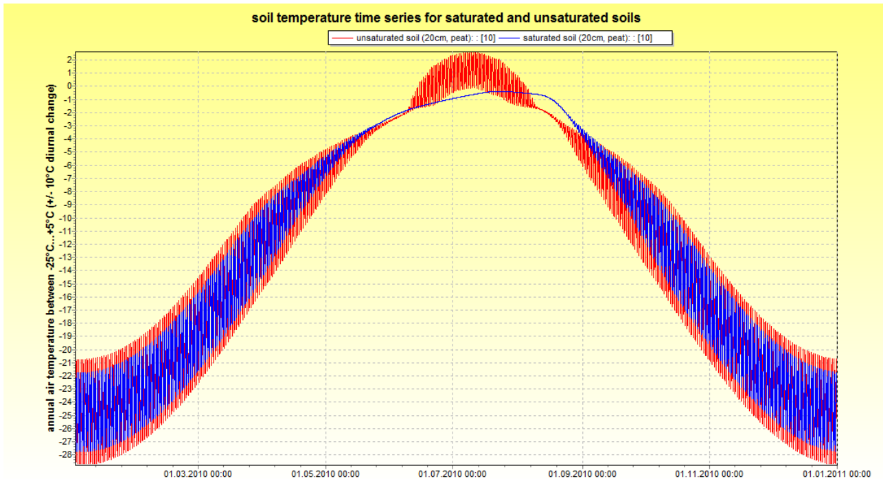
figure 2.25.8.13: Comparison of soil temperatures in 20 cm depth for a saturated (blue) and unsaturated (red) peat (porosity 0.8);
