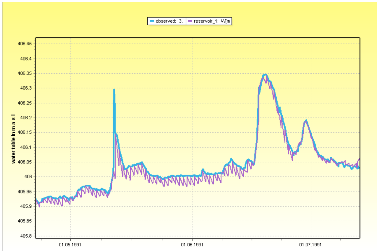
Abbildung 2.19.6: Comparison of modeled (purple) and observed water levels (blue) for lake Zurich with externally read abstraction values and with externally assimilated water table values (only once a day), zoom-in
