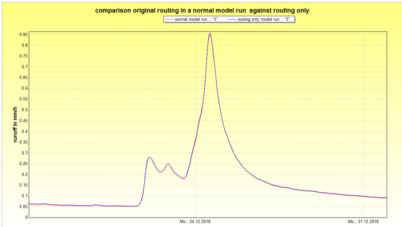
figure 2.17.3.2: Comparison between routing results for a normal model run (red) and a routing only model run (blue) with identical parameters; December 2018 flood event; Gauge Kander/Hondrich (491km 2 )
