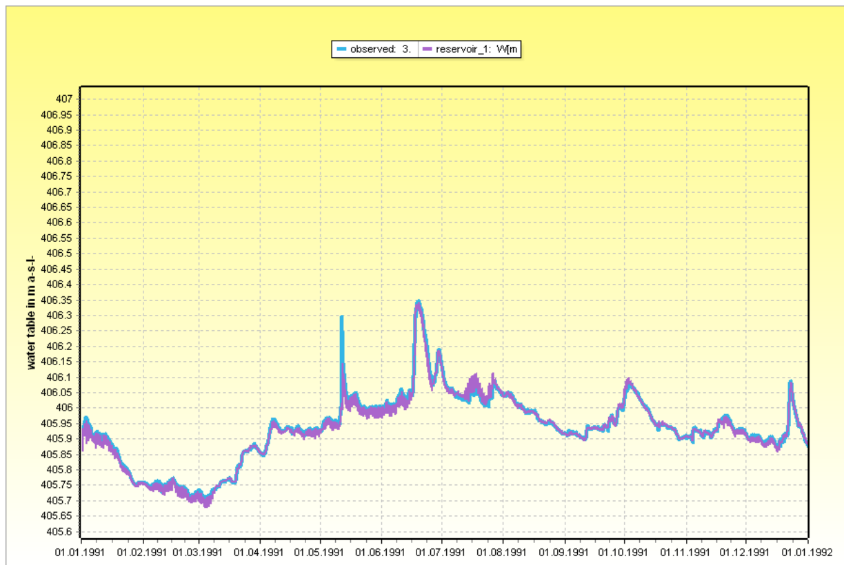
Abbildung 2.19.5: Comparison of modeled (purple) and observed water levels (blue) for lake Zurich with externally read abstraction values and with externally assimilated water table values (only once a day)
