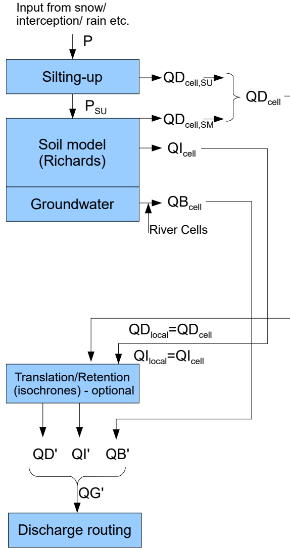
figure 2.13.2.4: Flow chart for soil- and routing modelling including silting-up but without surface routing
