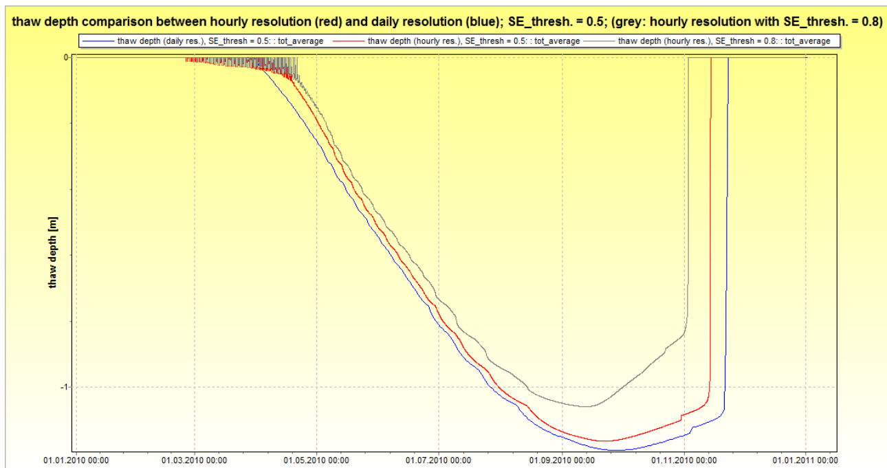
figure 2.25.8.5: Thaw depth for simulation in hourly and daily resolutions (red: hourly resolution with SE_{threshold} = 0.5 ; blue: daily resolution with SE_{threshold} = 0.5 ; grey: hourly resolution with SE_{threshold} = 0.8 )
