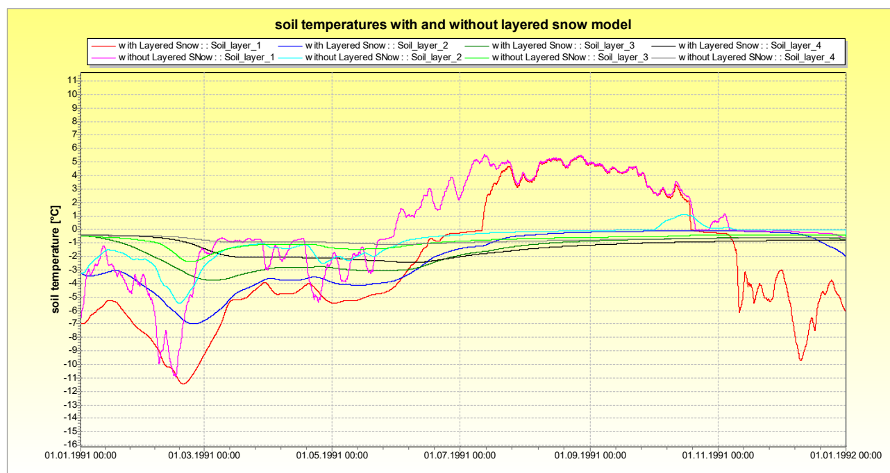
figure 2.27.3.1: soil temperatures for the first four soil layers (each 0.33m thick) with and without layered snow model
