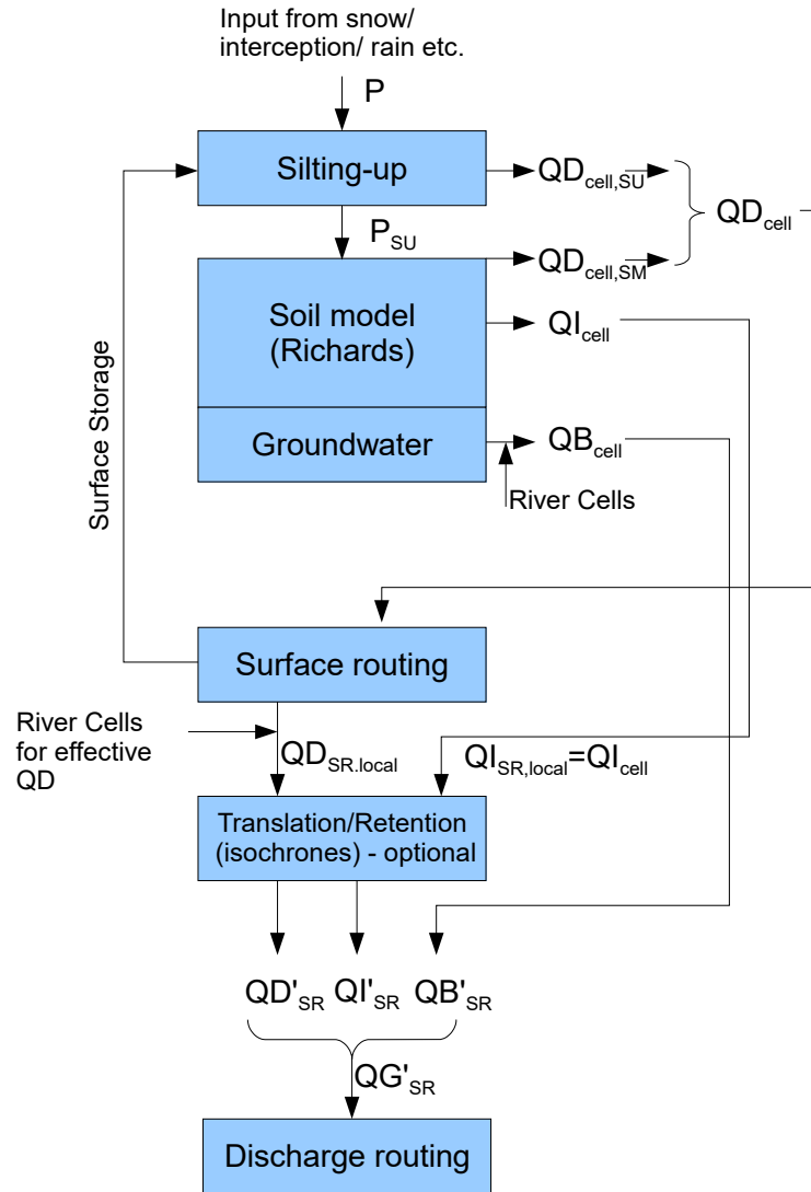
figure 2.13.2.2: Flow chart for soil- and routing modelling including silting-up and surface routing (starting from version 8.1.01)
