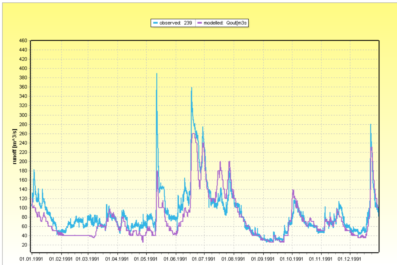
Abbildung 2.19.1: Comparison of modeled (purple) and observed runoff (blue) for lake Zurich without externally read abstraction values (purely modeled)
