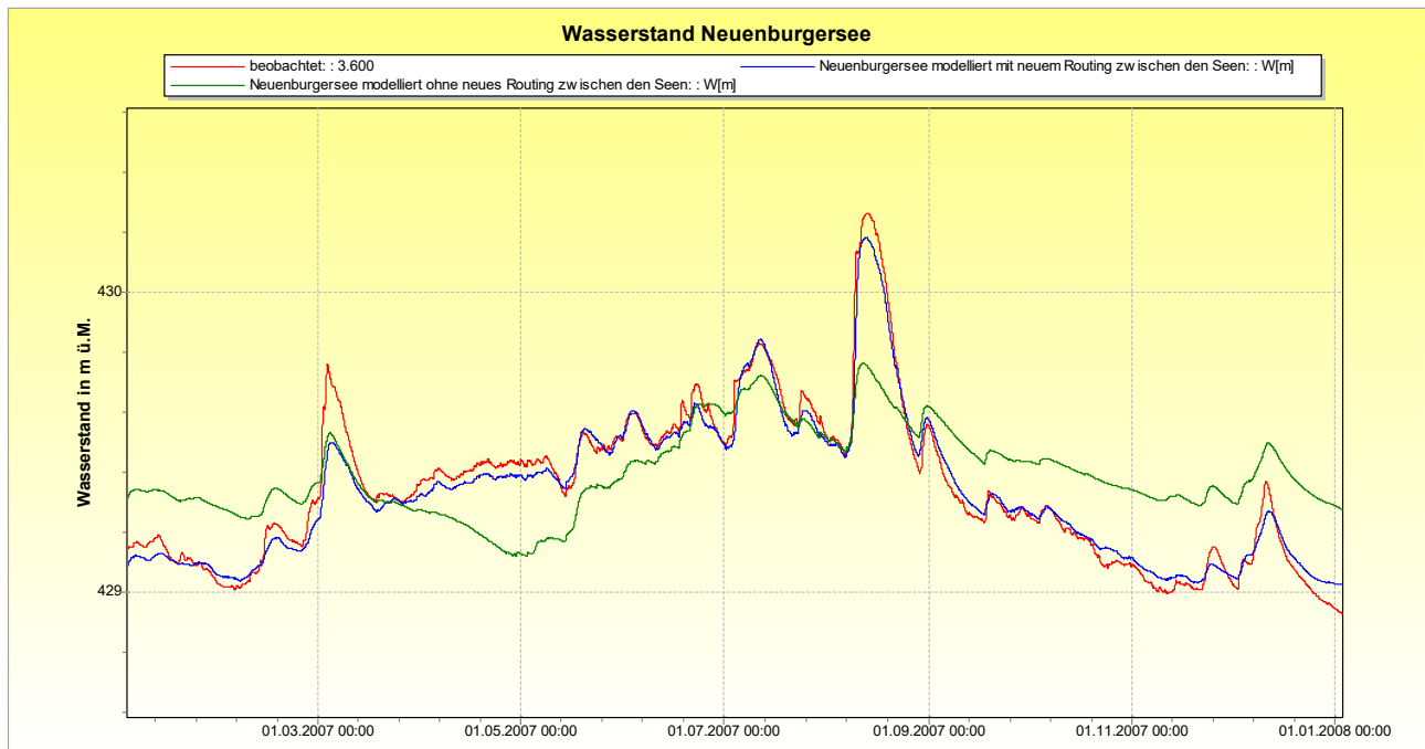
figure 2.19.9.3: Example for modeled lake water table with and without the new hydraulic connection abstraction rule (red=observed water table, green=modeled water table without hydraulic connection, i.e. classic one-way-routing, and blue=modeled water table with hydraulic connection)
