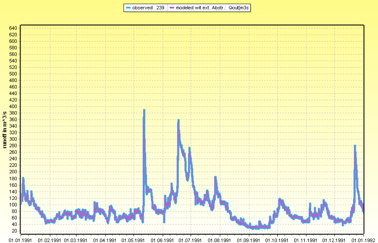
Abbildung 2.19.3: Comparison of modeled (purple) and observed runoff (blue) for lake Zurich with externally read abstraction values (only external values used)
