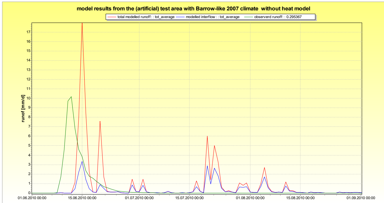
figure 2.25.8.6: Model results from an artificial arctic test site with a Barrow-like climate without the soil heat transfer model. The curves represent observed runoff (green), total modeled runoff (red), and modeled interflow (blue).
