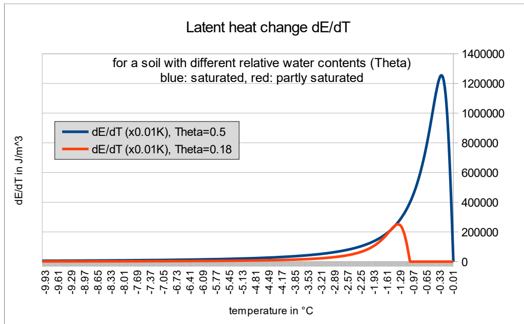
figure 2.25.5.1: The change in energy, i.e. latent heat, per temperature change of 0.01^{\circ}\text{C} for a soil with \Theta_s = 0.5 and \Theta_r = 0.1 for saturated (Theta=0.5) and unsaturated (Theta=0.18) conditions.
