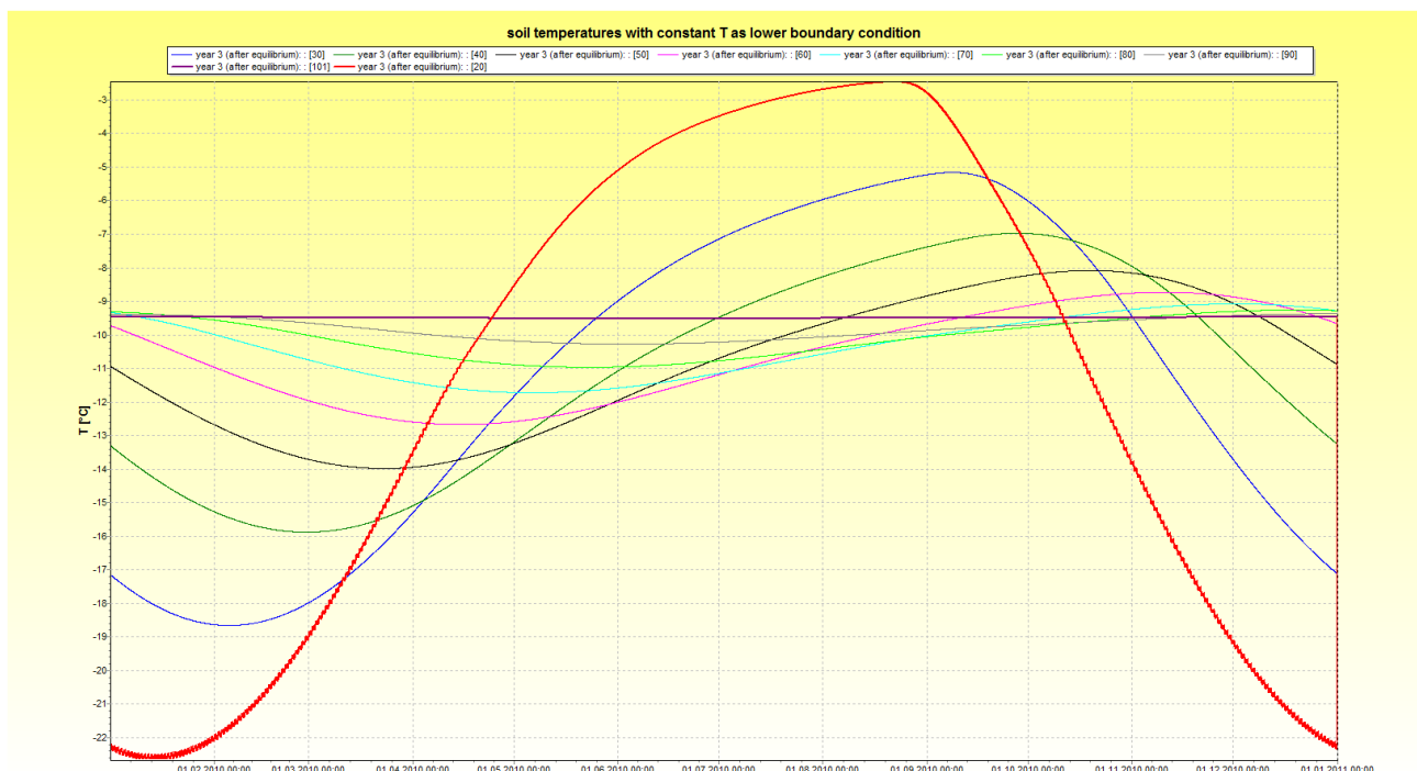
figure 2.25.8.9: soil temperatures as time series for constant T lower boundary condition (red=0.7m, blue = 1.7m, green = 2.7m, black = 3.7m etc. down to 8.8m for violet)
