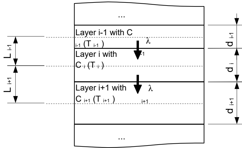
figure 2.25.7.1: Definition of layer indices for the discrete 1D heat transfer model describing heat transfer through conduction.
