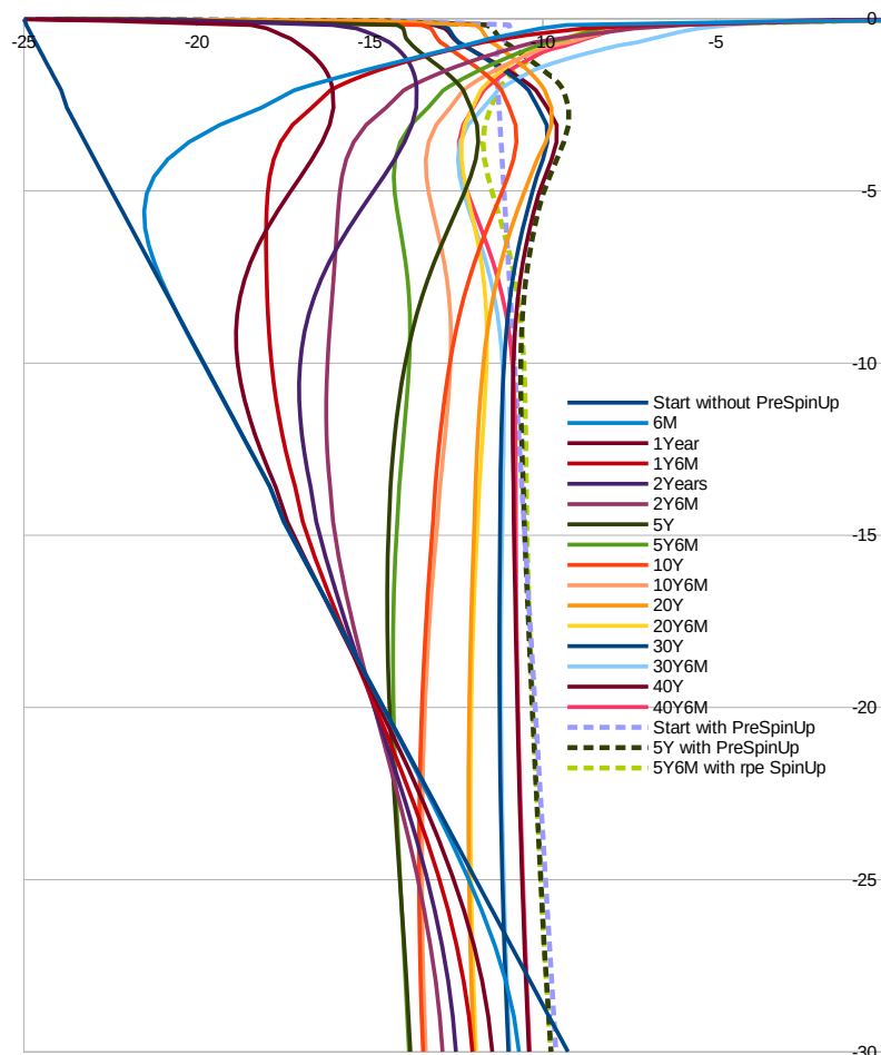
figure 2.26.4.1: soil temperature profiles without pre-spin-up (solid lines) and with pre-spin-up (dashed lines)
