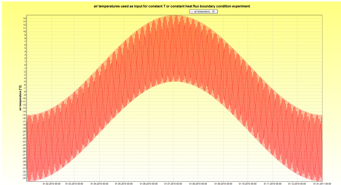
figure 2.25.8.8: air temperature for the following experiments. T ranges from -25^{\circ}\text{C} in winter to +5^{\circ}\text{C} in summer with diurnal fluctuations of \pm 10^{\circ}\text{C} . Annual average is -10^{\circ}\text{C}
