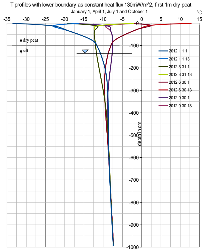
figure 2.25.8.18: T-profiles for unsaturated soil
