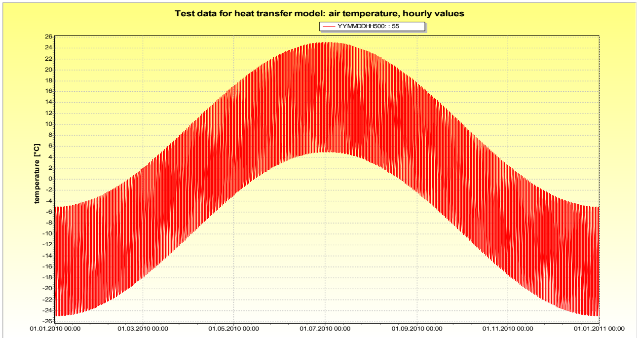
figure 2.25.8.1: temperatures used for heat transfer test data for hourly data (daily fluctuation \pm 10^{\circ}\text{C} )
