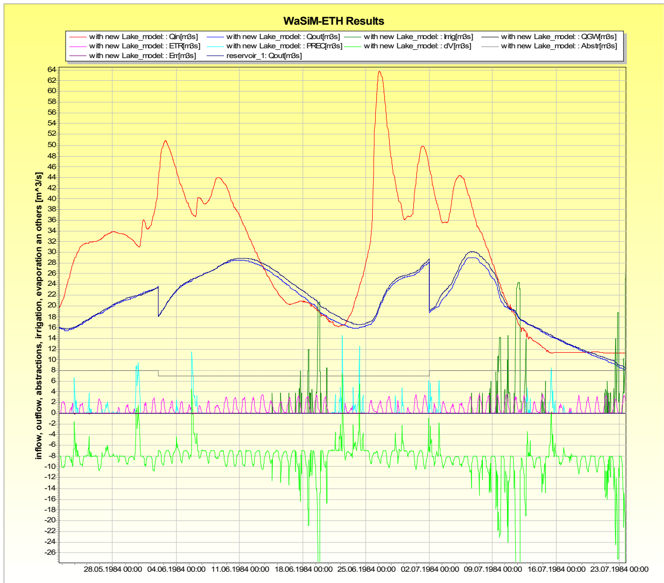
figure 2.19.10.2: some components of the lakes water balance statistics.
