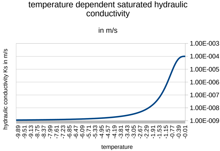
figure 2.25.4.2: Effective hydraulic conductivity using an exponential function (Eq. 2.24.8b).
