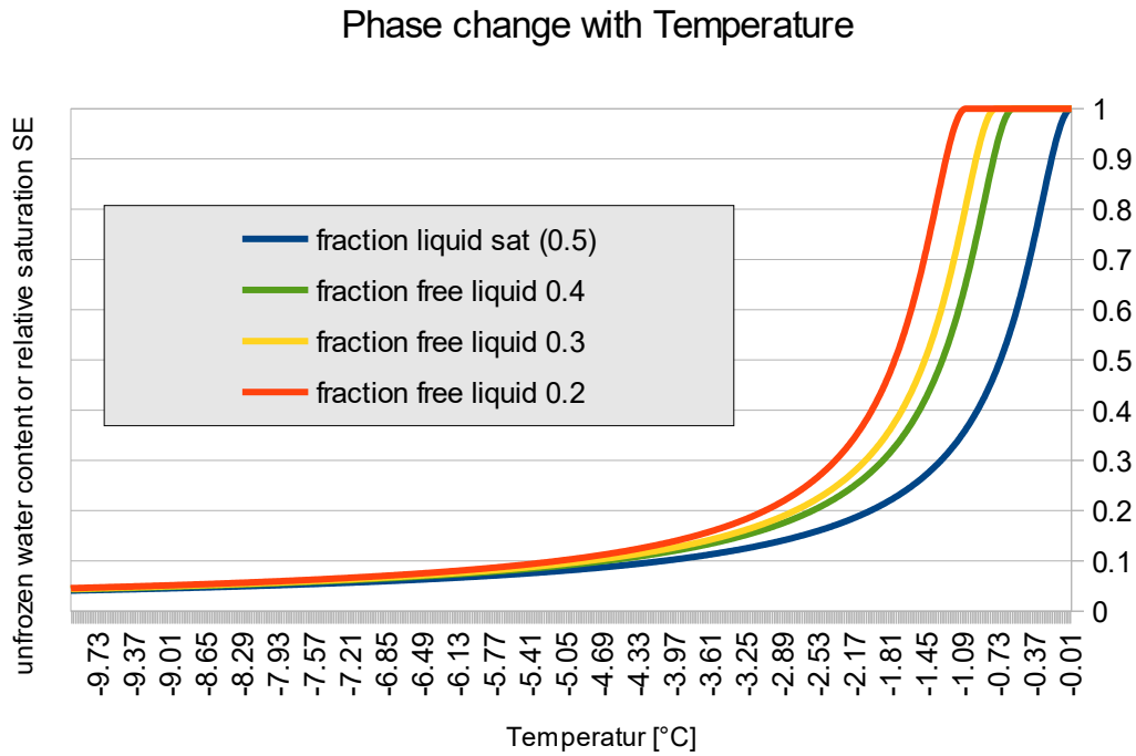
figure 2.26.2.1: Change in the fraction of liquid water, S_E , during temperature change in a sandy loam soil ( \alpha=2 , n=2 , m=0.5 ). (temperatures are negative from -10 to 0°C)
