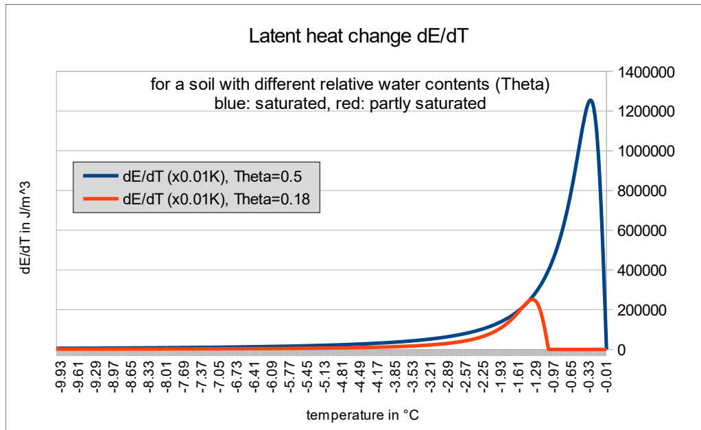
figure 2.26.5.1: The change in energy, i.e. latent heat, per temperature change of 0.01^{\circ}\text{C} for a soil with \Theta_s = 0.5 and \Theta_r = 0.1 for saturated ( \Theta = 0.5 ) and unsaturated ( \Theta = 0.18 ) conditions.
