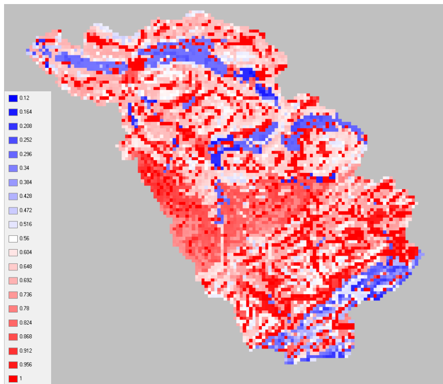
figure 2.30.5.2: spatial distribution of relative soil moisture for January, 7th, 1991, Thur basin
