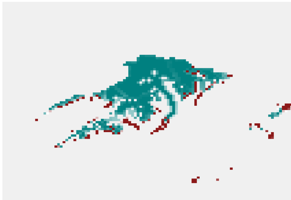
figure 2.23.2.2: Glaciers in the Swiss Alps for 2010
