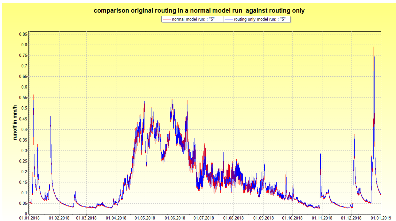
figure 2.18.3.3: Comparison between routing results for a normal model run (red) and a routing only model run (blue) with different roughness parameters; 2018, Gauge Kander/Hondrich (491km 2 )
