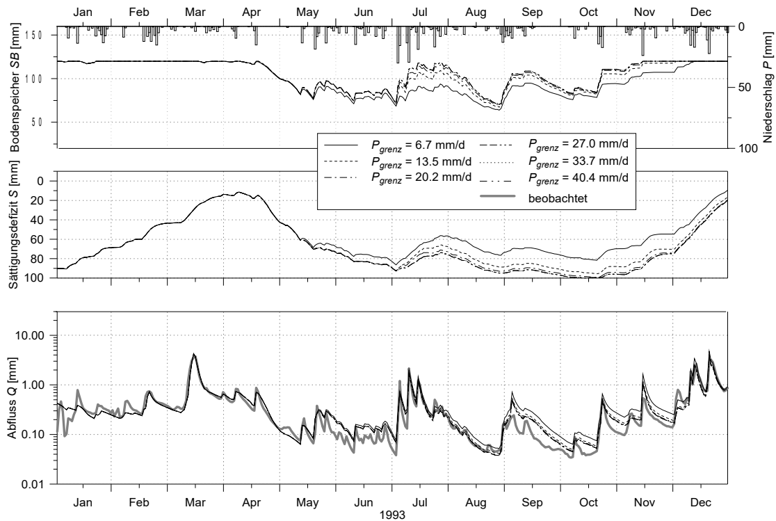
figure 4.15.5.5: Impact of the threshold precipitation intensity P_{\text{grenz}} for generating macro pore drainage on (a) soil moisture, (b) saturation deficit and (c) runoff; without capillary rise/reflow from interflow into soil storage ( r_k = 0.0 ); Wernersbach, Saxonia, 4.6 km 2 , 365 to 465 m ü.M., daily time steps for 1993; “Abfluss”=discharge, “Sättigungsdefizit”=saturation deficit, “Bodenspeicher”=soil storage, “beobachtet”=observed
