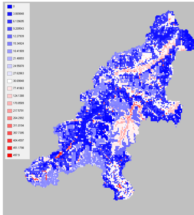
figure 2.30.2.3: actual field capacity 1991-01-31 in mm
