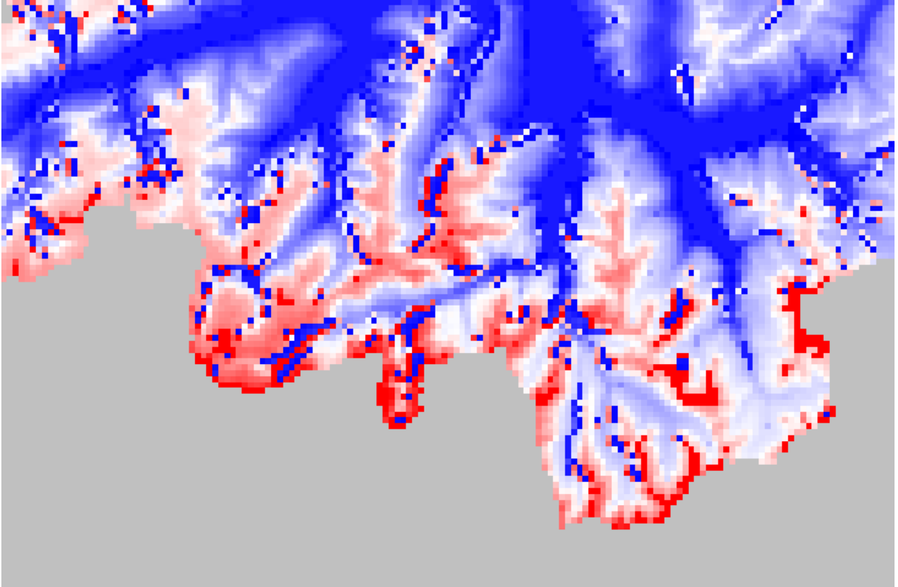
figure 2.9.4.2: snow distribution pattern with slides (in mm SWE)
