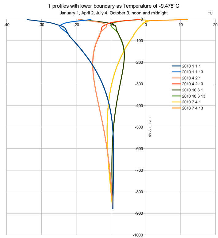
figure 2.26.8.11: T-Profile with constant T - 9.478^{\circ}\text{C} as lower boundary condition
