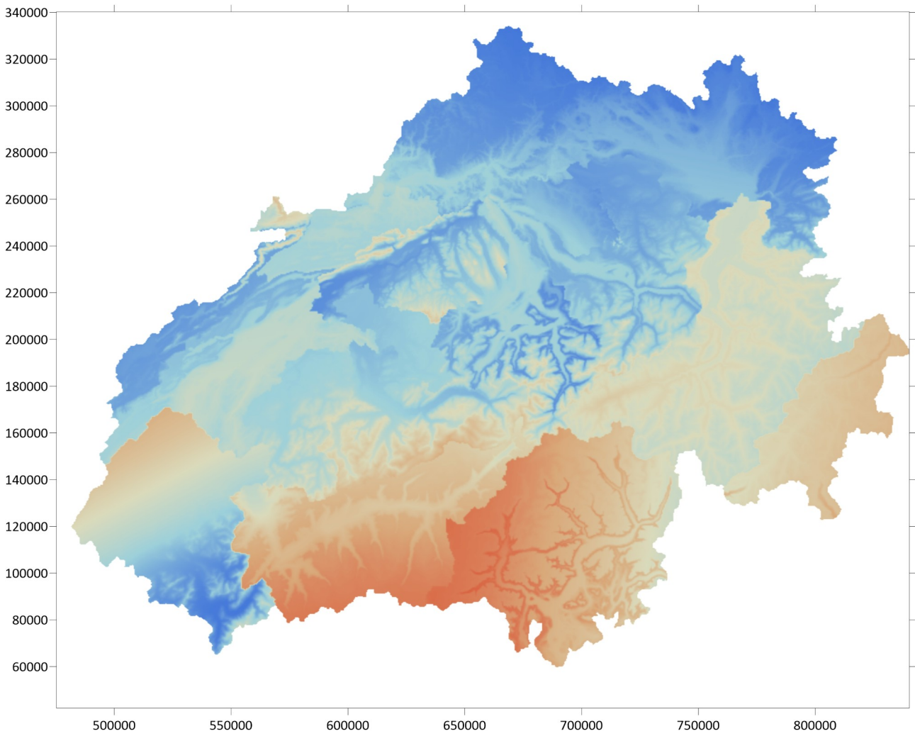
figure 2.30.1.1: Example of relative air humidity interpolation results for all Swiss river basins, interpolated independently of each other
