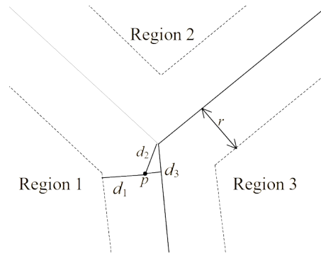
figure 2.3.13.1: Weighting of multiple regions for a point p near the regions crossing point
