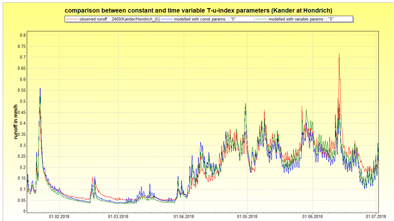
figure 2.10.3.1: comparison of modeled runoffs versus observed runoff (red) for blue=constant T-u-index parameters and green = temporally variable parameters
