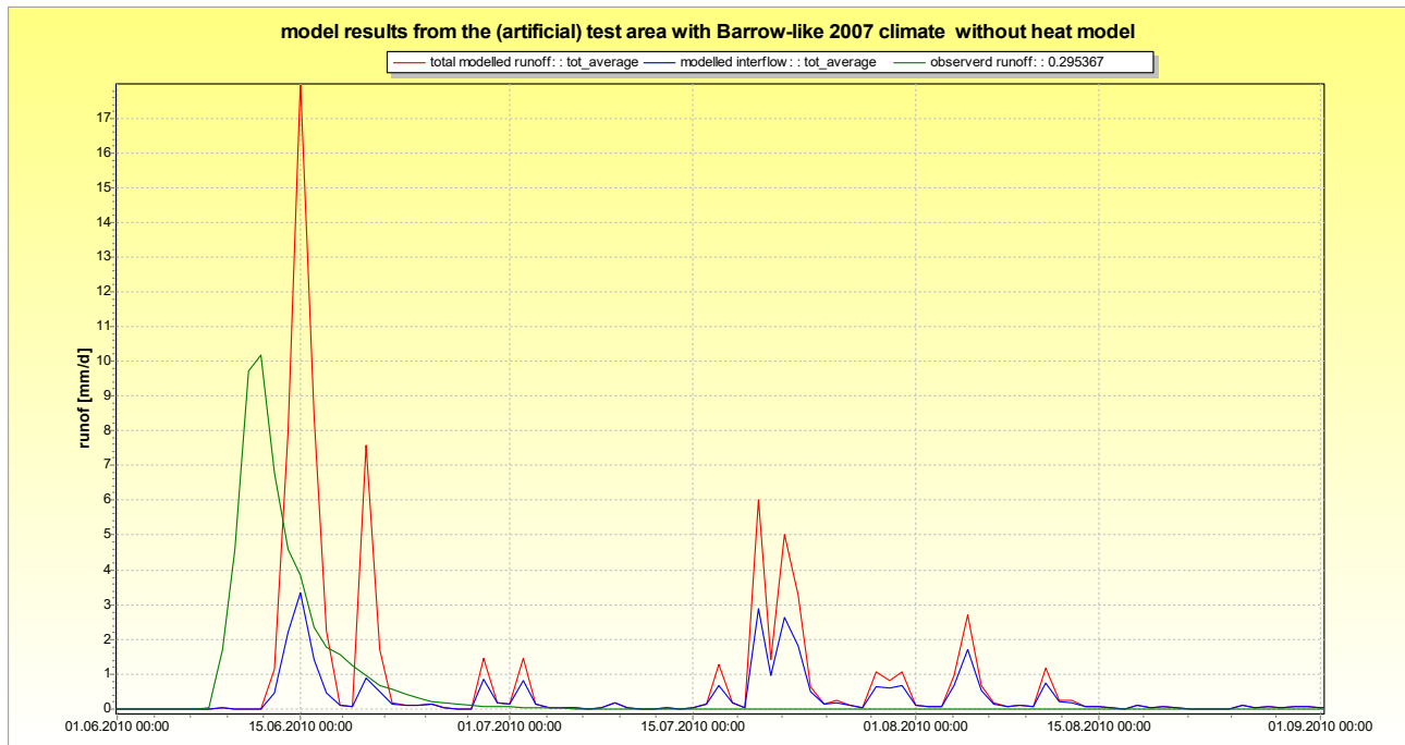
figure 2.26.8.6: Model results from an artificial arctic test site with a Barrow-like climate without the soil heat transfer model. The curves represent observed runoff (green), total modeled runoff (red), and modeled interflow (blue).
