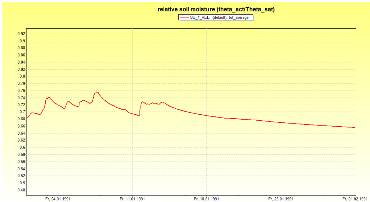
figure 2.30.5.1: statistics for relative soil moisture for the river Thur basin, January 1991
