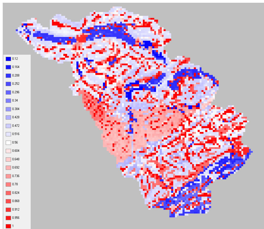
figure 2.30.5.3: spatial distribution of relative soil moisture for January, 31st, 1991, Thur basin
