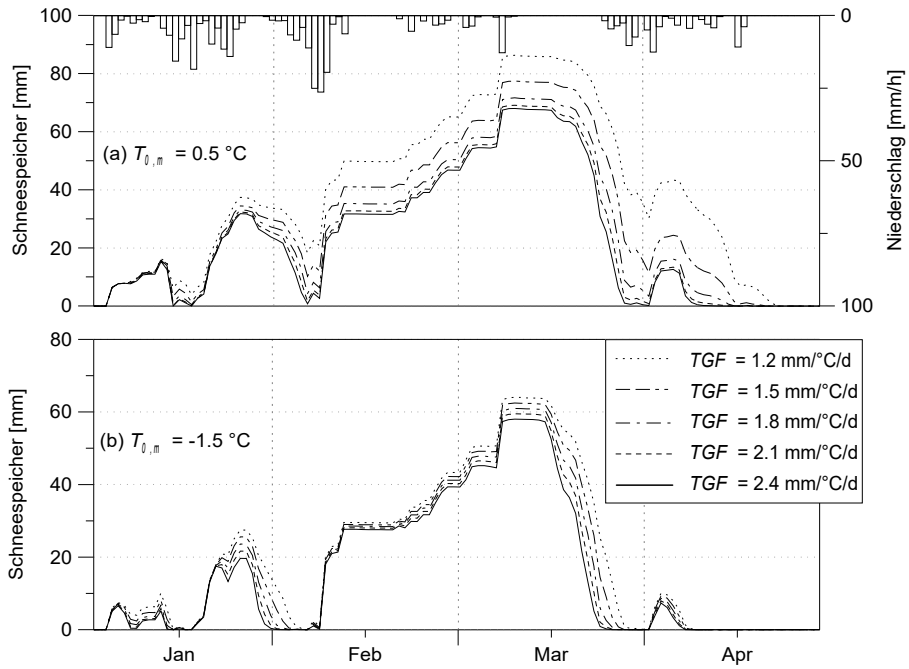
figure 4.15.4.2: temporal course of snow water equivalent for different degree day factors: (a) melt threshold temperature T_{0,m} = +0.5 °C, (b) T_{0,m} = -1.5 °C, Rietholzbach basin, 1984; “Schneespeicher” means snow water equivalent, “Niederschlag” means precipitation
