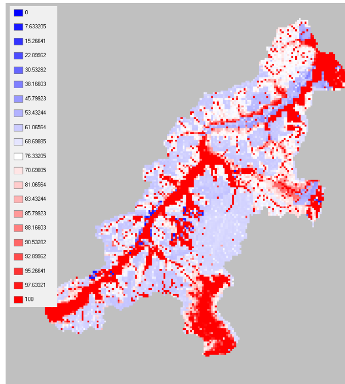
figure 2.30.2.4: actual water content 1991-01-31 as percentage of actual content on field capacity (in %)
