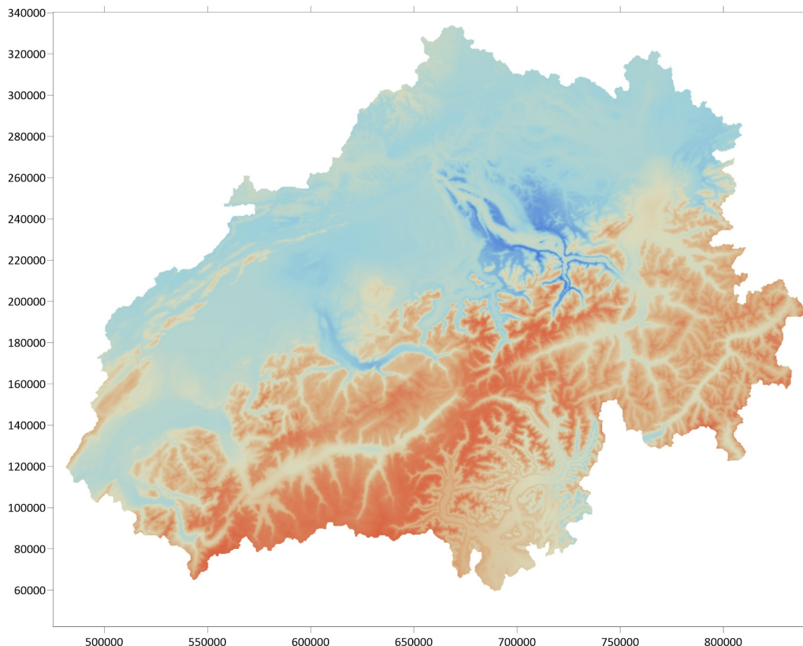
figure 2.30.1.2: Example of relative air humidity interpolation results for all Swiss river basins, interpolated independently of each other but with smooth shifts between regions
