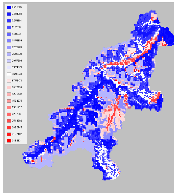
figure 2.30.2.2: Maximum usable field capacity in mm
